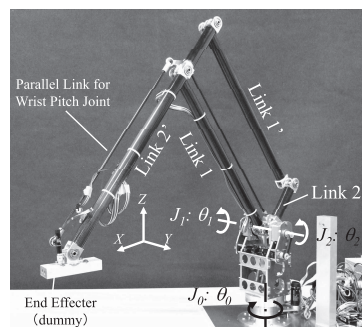
Fig. 14 Prototype model of a parallel four-bar linkage arm for a light duty operation
