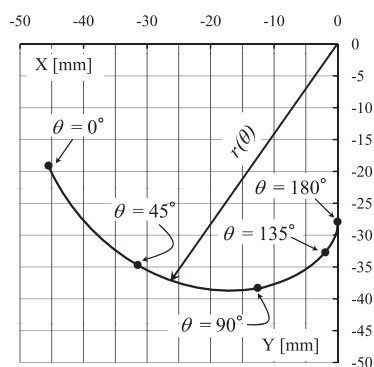
Fig. 4 An example of the Non-circular Pulley
