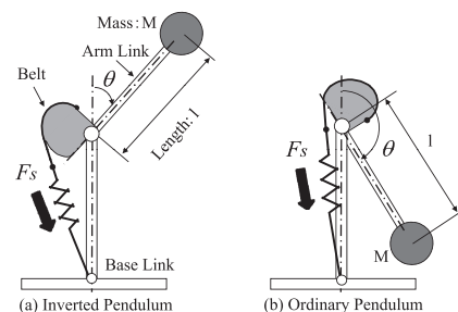
Fig. 2 Weight compensation mechanism with a non-circular pulley and a spring
