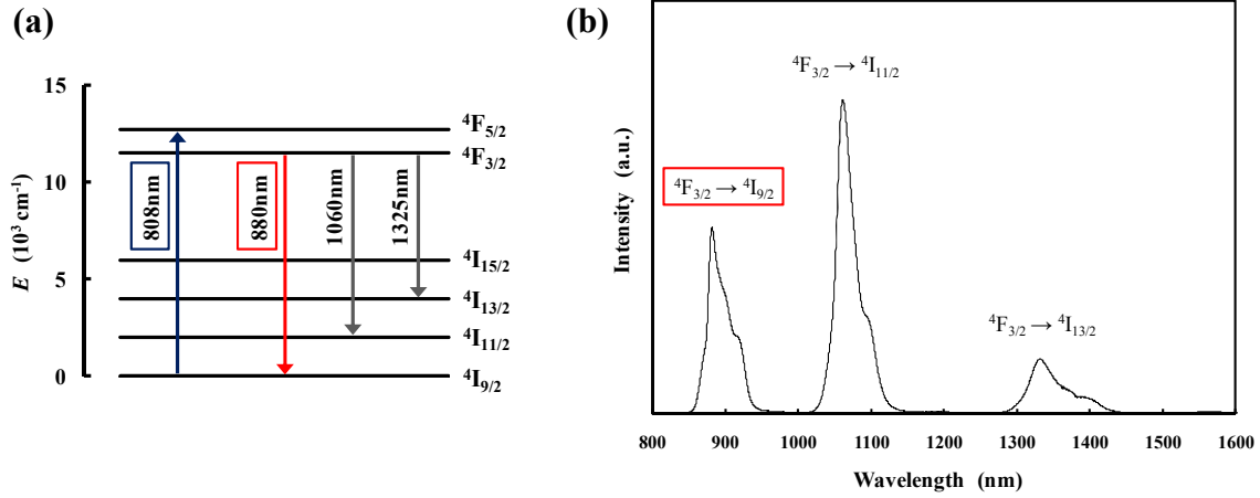
Fig. 8. (a) Energy level diagram of Nd^{3+} ion. Arrow lines show laser transition processes. (b) Fluorescent spectrum of Nd-doped soda-lime silica glass (excitation wavelength is 810nm).
