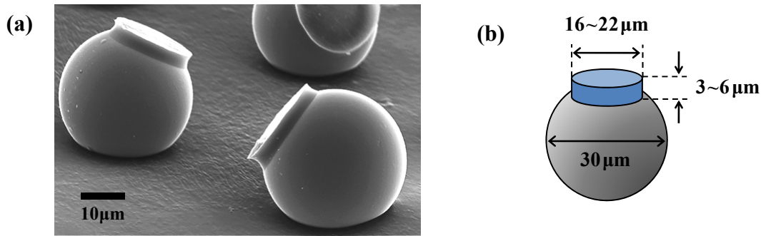
Fig. 3. (a) SEM image of terrace-microspheres. (b) Schematic illustration of a terrace-microsphere.
