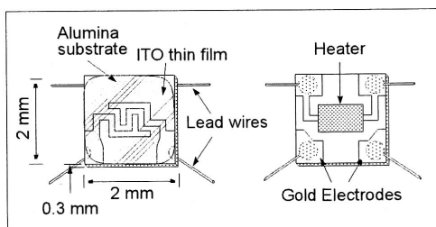
Fig. 1 Sensing Elements
