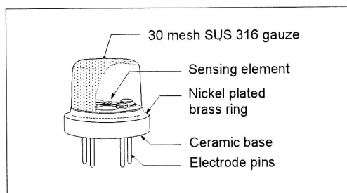
Fig. 2 Structure
