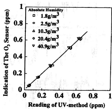
Fig. 6 Correlation between indication of the present \text{O}_3 sensor after the absolute humidity compensation and reading of the UV-method.
