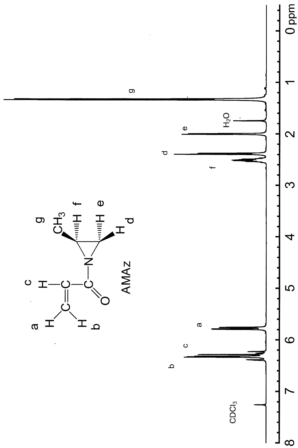
Figure 2-2-4. ^1\text{H} NMR Spectrum of AMAZ.
