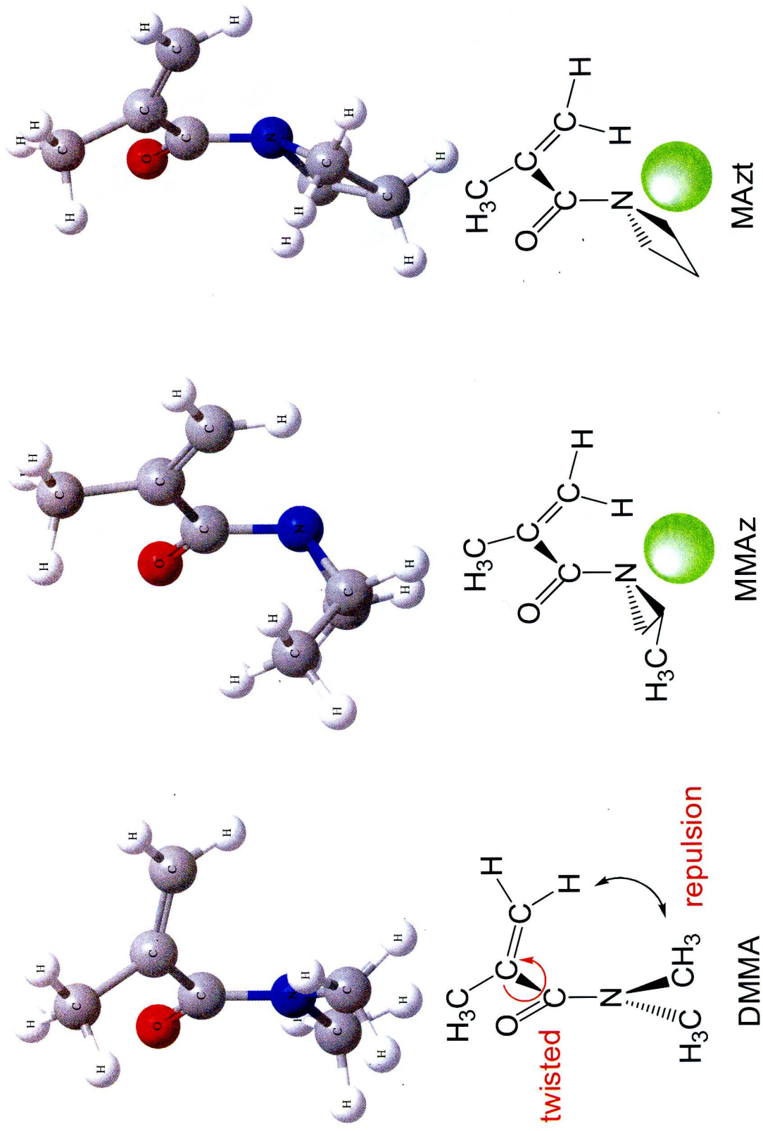
Figure 4-4 Conformation of MMA, MMAz, and MAzt.
