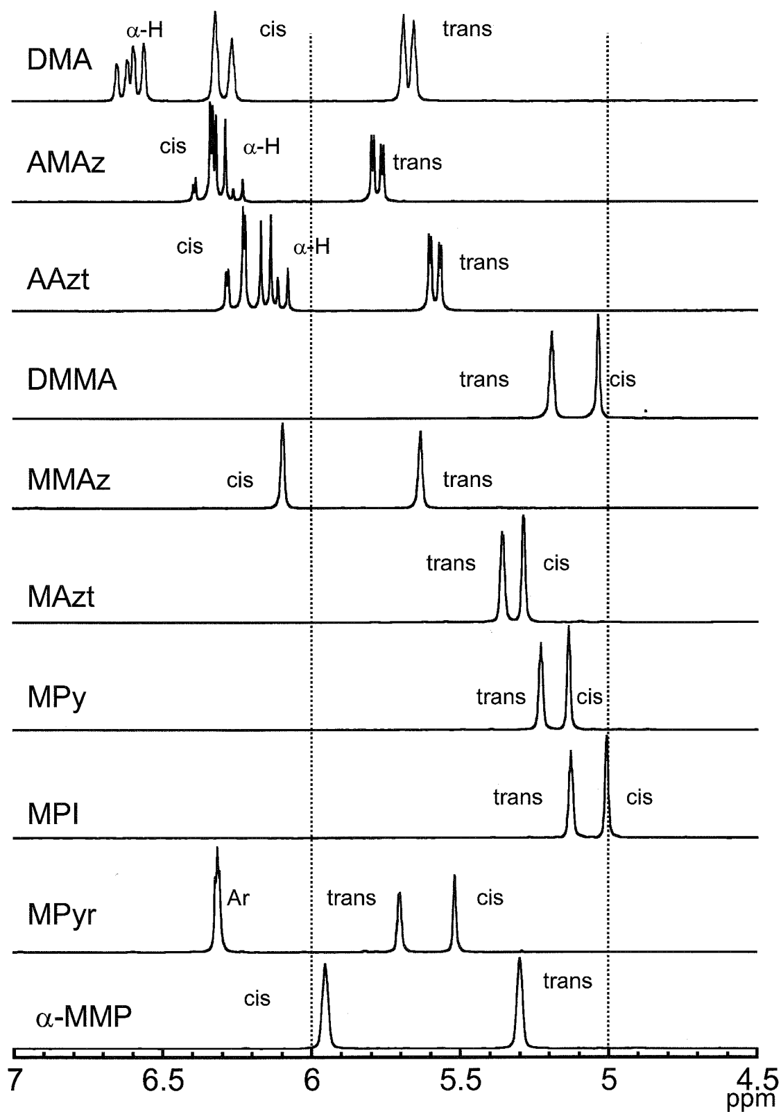
Figure 4-1. ^1\text{H} NMR Spectra of N,N -Dialkyl(meth)acrylamides at Vinyl Group Region.
