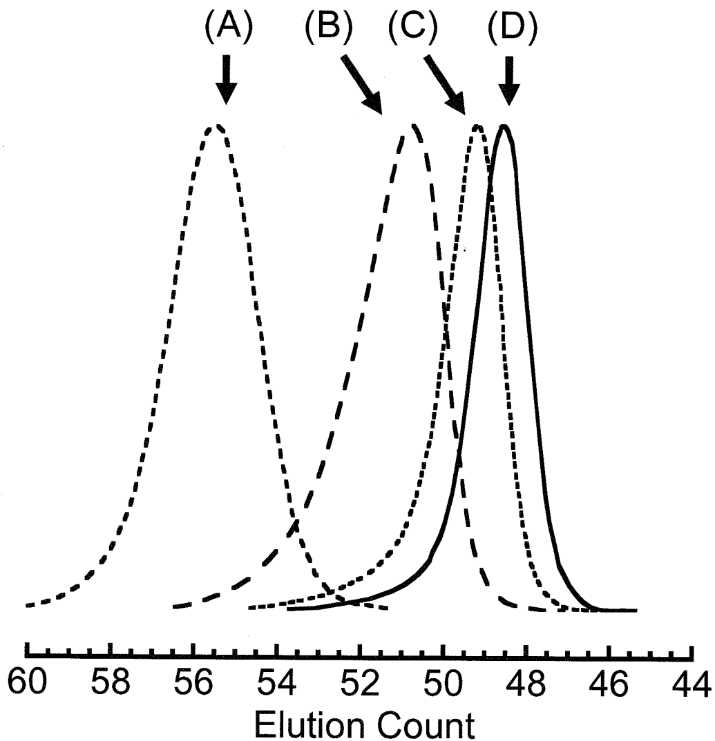
Figure 3-3-14. GPC curves of a series of poly(MAzt)s obtained with DMPLi and 4.6-fold LiCl in THF at -40^{\circ}\text{C} .
