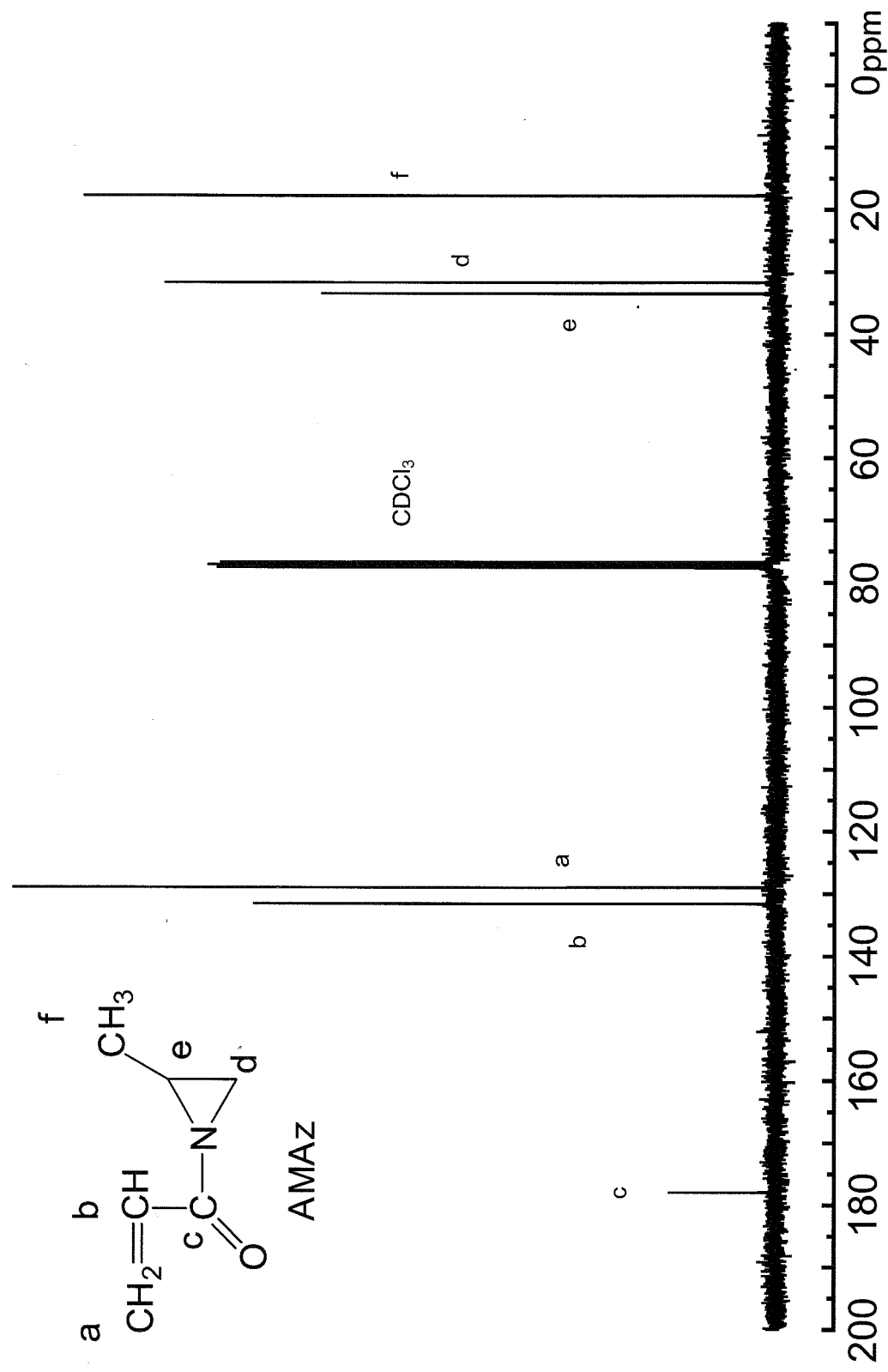
Figure 2-2-5. 13 C NMR Spectrum of AMAZ.
