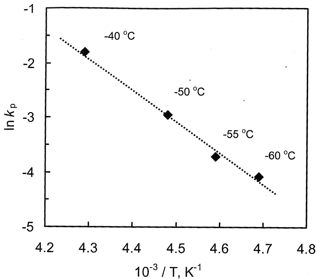
Figure 2-4-13. Arrhenius plots of k_p for the polymerization of MMAz with DMPLi and 4.4-4.9-fold LiCl om THF.
