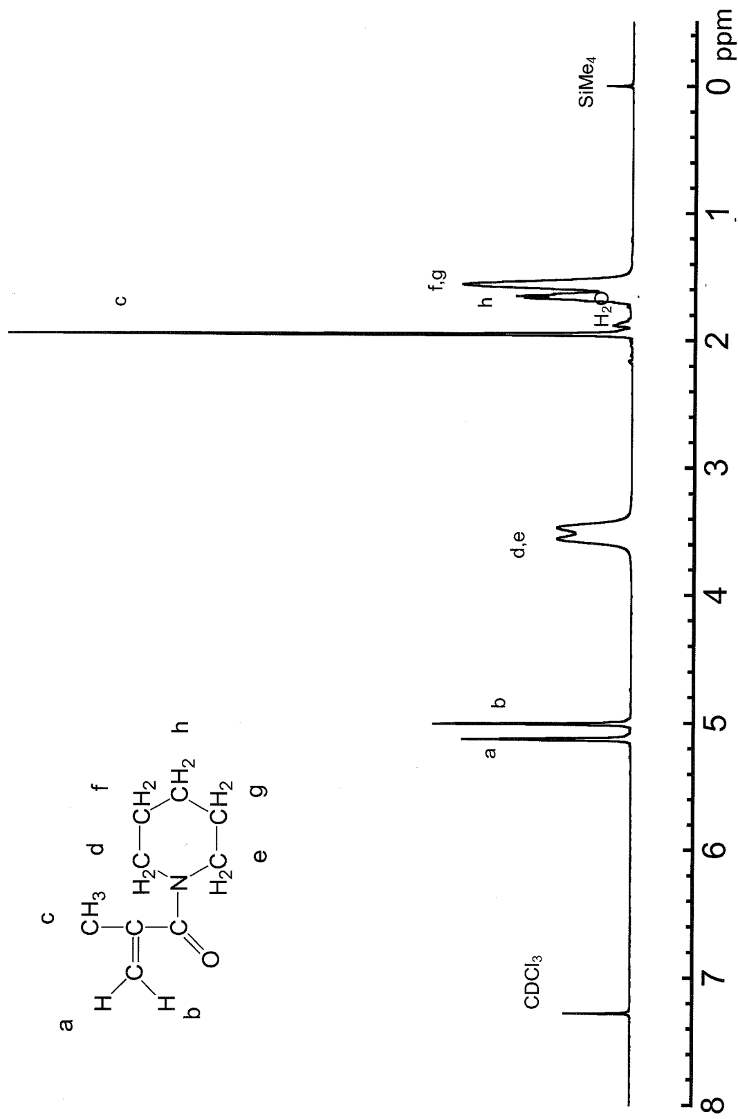
Figure 3-2-10. ^1\text{H} NMR Spectrum of MPI.
