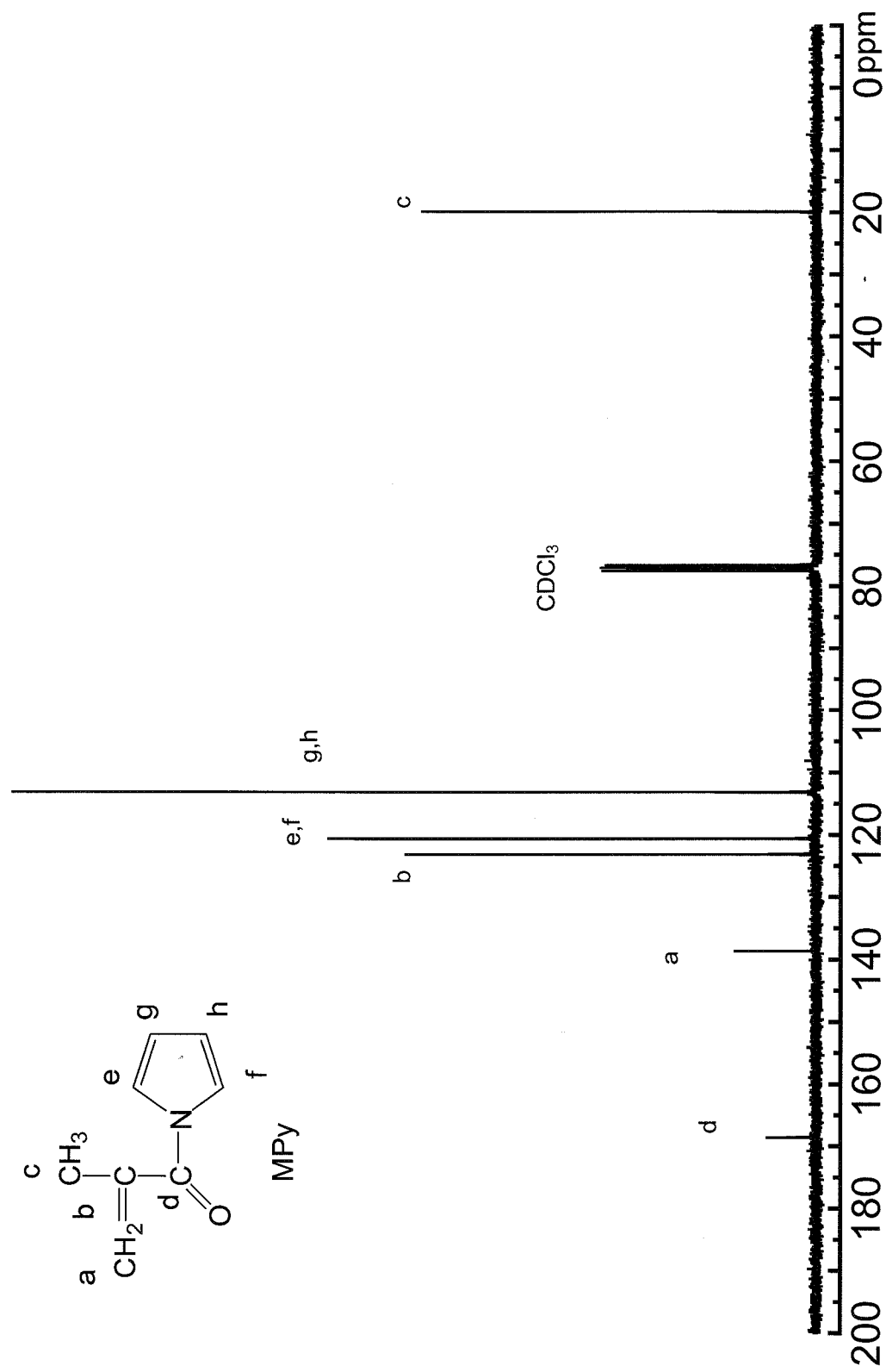
Figure 3-2-14. ^{13}\text{C} NMR Spectrum of MPy.
