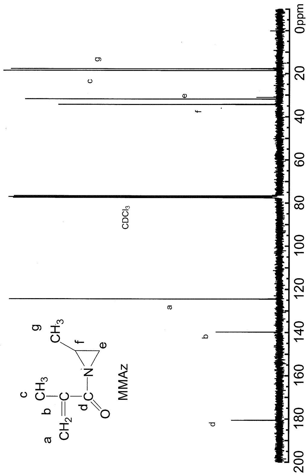
Figure 2-2-2. 13 C NMR Spectrum of MMAZ.
