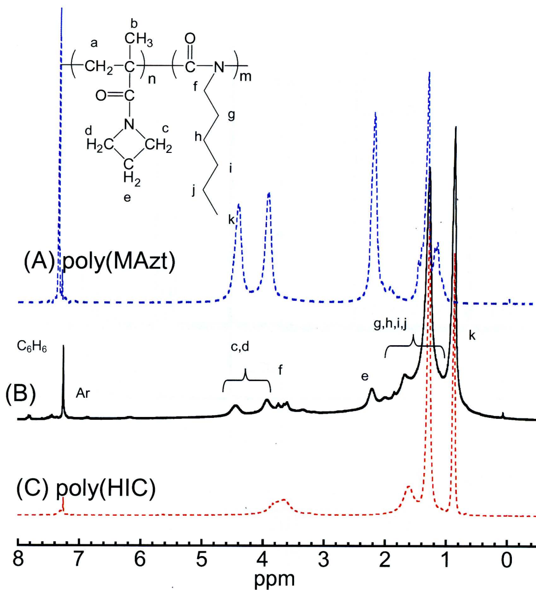
Figure 3-3-11. ^1\text{H} NMR Spectra of Poly(MAzt)- b -poly(HIC).
