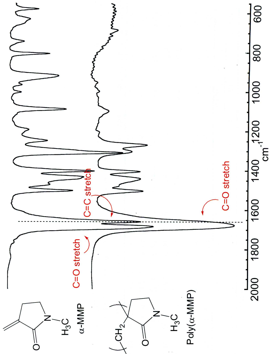
Figure 3-8-3. IR Spectra of \alpha -MMP and Poly( \alpha -MMP).
