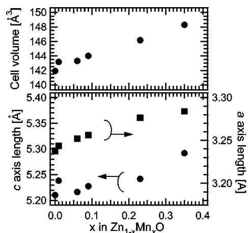
FIG. 1. Mn content dependence of cell volume (top) and a - and c -axes lattice constants (bottom) for \text{Zn}_{1-x}\text{Mn}_x\text{O} films.
