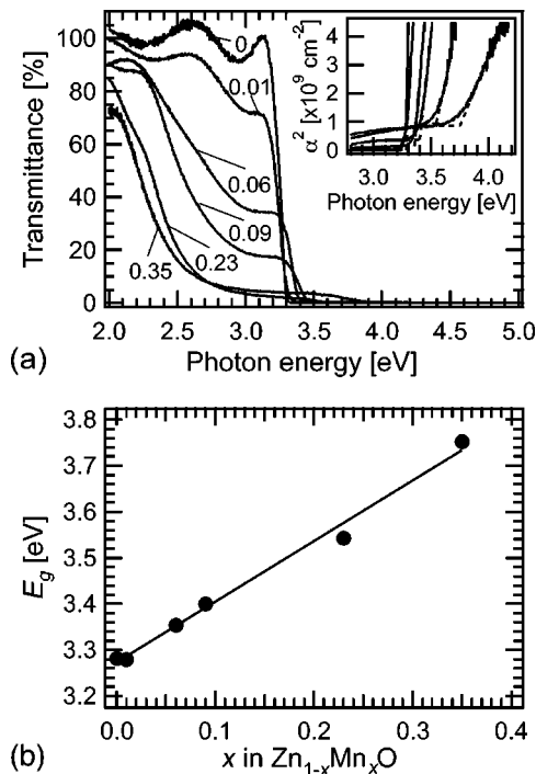
FIG. 2. (a) Transmittance spectra of \text{Zn}_{1-x}\text{Mn}_x\text{O} films measured at room temperature for various x values. Numbers in the figure denote x . Inset: Photon energy dependence of \alpha^2 for deducing band gap ( E_g ) from the intersection of the dotted lines. (b) Variation of E_g with Mn content. The solid line is a fitted line expressed as E_g = 3.273 + 1.32x [eV].
