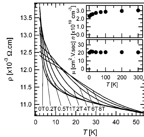
FIG. 3. Temperature dependence of resistivity in various magnetic fields for a \text{Zn}_{0.81}\text{Mn}_{0.19}\text{O}:\text{Al} film. Inset: Temperature dependence of carrier concentration (top) and mobility ( \mu ) (bottom).
