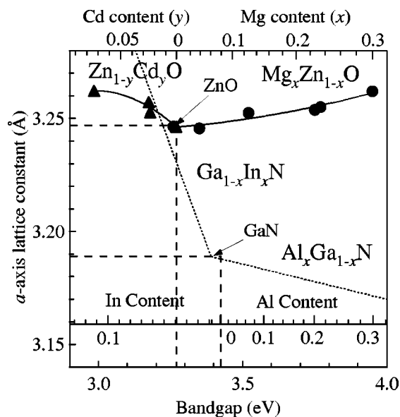
FIG. 3. Optical and structural properties of \text{Cd}_y\text{Zn}_{1-y}\text{O} and \text{Mg}_x\text{Zn}_{1-x}\text{O} alloy films mapped out in a plane of a-axis length and room-temperature band gap energy. The curves for (In,Ga)N and (Al,Ga)N alloys are also shown. Alloy compositions are shown at the top axis.
