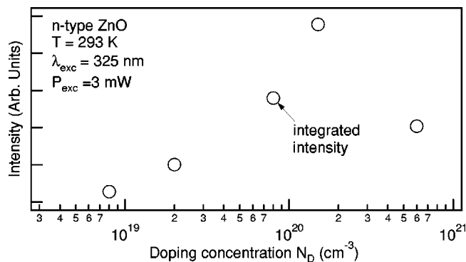
FIG. 2. Integrated emission intensity of the near-band-edge transition of n -type ZnO as a function of the doping concentration.
