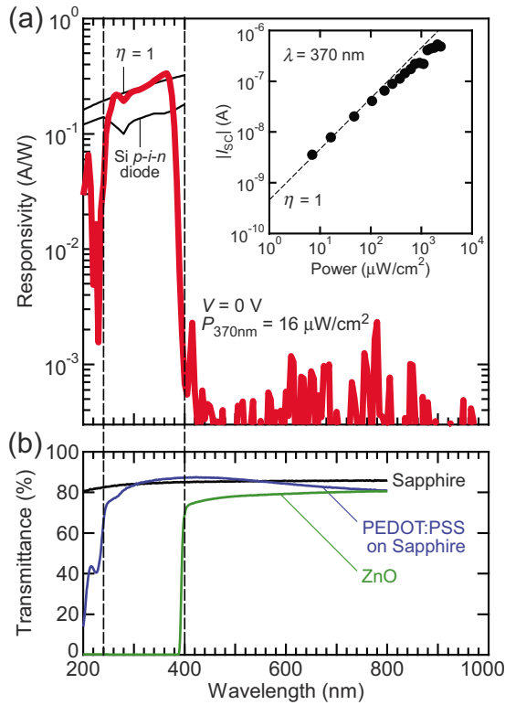
FIG. 3. (Color online) (a) The spectral response of the PEDOT:PSS/ZnO Schottky photodiode at V=0 V and P_{370\text{ nm}}=16\text{ }\mu\text{W}/\text{cm}^2 . That of the Si p - i - n photodiode and a spectrum corresponding to a quantum efficiency ( \eta ) of unity are also indicated for comparison. The inset shows the incident light power ( P_\lambda ) dependence of the short-circuit current ( I_{sc} ) at \lambda=370 nm with the dashed line representing \eta=1 . (b) Transmission spectra of a sapphire, a 50-nm-thick PEDOT:PSS thin film on a sapphire, and a ZnO single crystal substrate.
