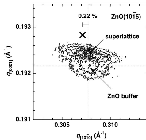
FIG. 3. X-ray diffraction reciprocal space contour map around (1015) diffraction for a superlattice sample with L_W = 12 nm. The buffer ZnO layer and superlattice have an identical q[1010] value, indicating the barrier \text{Mg}_{0.2}\text{Zn}_{0.8}\text{O} layer is strained to form a pseudomorphic epitaxial structure. The cross in the figure is the peak position for a thick \text{Mg}_{0.2}\text{Zn}_{0.8}\text{O} film. The lattice mismatch is as small as 0.22%.
