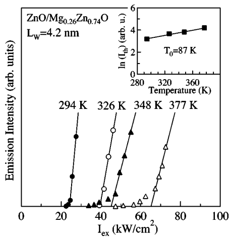
FIG. 4. Temperature dependence of the emission intensity as a function of excitation intensity ( I_{\text{ex}} ) in a \text{ZnO}/\text{Mg}_{0.26}\text{Zn}_{0.74}\text{O} SL ( L_w = 4.2 nm). The inset shows the threshold intensity ( I_{\text{th}} ) as a function of temperature on a logarithmic scale.
