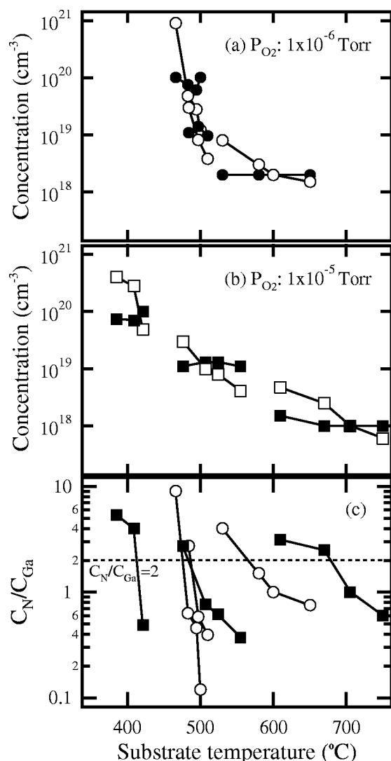
FIG. 10. Temperature dependence of C_N and C_{Ga} in ZnO:(Ga,N) films deposited with (a) P_{O_2} : 1 \times 10^{-6} Torr and (b) 1 \times 10^{-5} Torr, using the temperature gradient method. The closed and open symbols represent C_{Ga} and C_N , respectively. (c) C_N/C_{Ga} ratio for the samples deposited with P_{O_2} : 1 \times 10^{-6} and 1 \times 10^{-5} Torr represented by open circle and closed square symbols, respectively. All specimens have a position where C_N/C_{Ga} = 2 .
