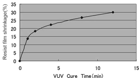
Fig. 1 Resist film shrinkage by VUV cure.
