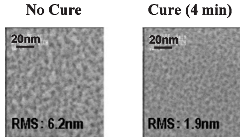
Fig. 5 Surface roughness of resist after dry etching with and without VUV cure.
