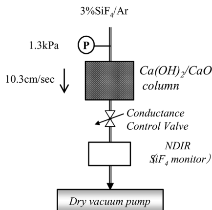
Fig. 3. Schematic diagram of experiment to evaluate the reactivity of \text{Ca}(\text{OH})_2/\text{CaO} .
