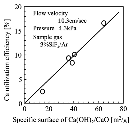
Fig. 6. Specific surface area dependence of reaction efficiency.
