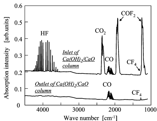
Fig. 7. Infrared absorption spectra at the inlet and outlet of the \text{Ca(OH)}_2/\text{CaO} column.
