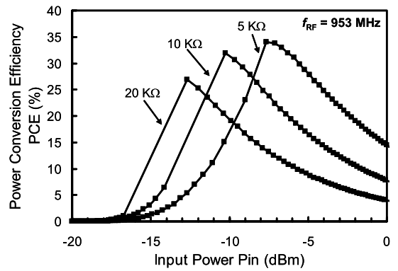
Fig. 12 Output load resistance R_L dependency on PCEs.
