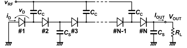
Fig. 1 Conventional rectifier circuit for RFIDs.
