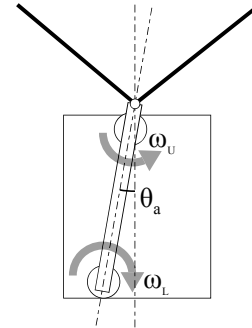
Fig. 17. Model of Clamping for the Sideways Drive.
