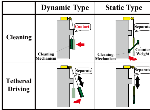
Fig. 2. Comparison of the Tethered Driving on the Wall.
