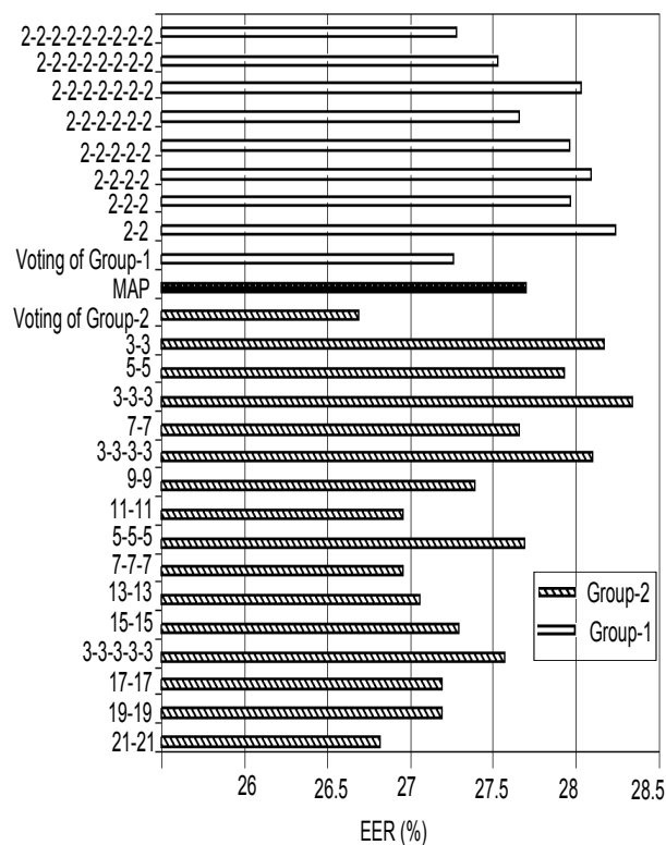
Fig. 2 EER for GMM-SVM systems using MAP and SMAP adaptation on the 10sec4w-10sec4w task of 2006 NIST SRE. The design of a tree is written as n_1 - n_2 - \dots - n_l where n_l represents the maximum number of child nodes belonging to each node of the l -th layer.
