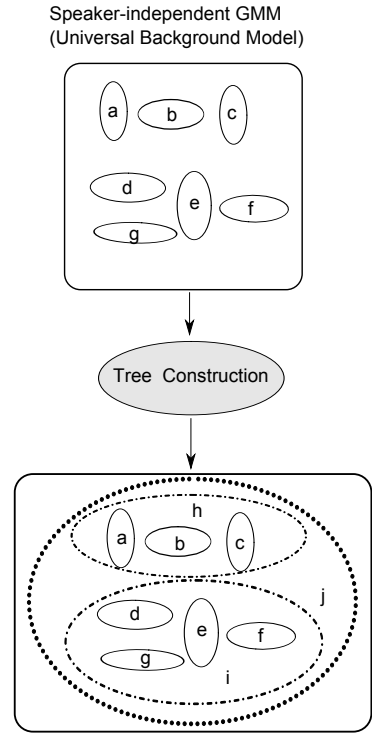
Fig. 1 Example of a tree structure of Gaussian components in SMAP. Each of a, b, \dots, g is Gaussian component of UBM. h, i and j are parent Gaussians of \{a, b, c\} , \{d, \dots, g\} and \{h, i\} , respectively.
