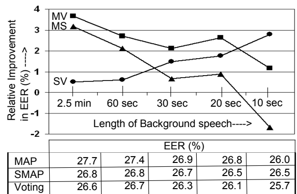
Fig. 3 Relative improvement in EER (%) for different length of speech segments of background speakers for three cases: (i) SV: Voting approach over SMAP, (ii) MV: Voting approach over MAP and (iii) MS: Best single tree based SMAP over MAP
