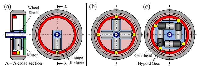
Fig. 3 Conventional low-profile arrangement
