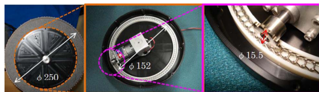
Fig. 6 Developed low-profile in-wheel motor
