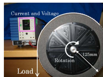
Fig. 7 Efficiency Measurement
