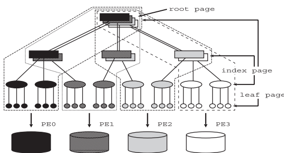
Fig. 1 A fat-btree.
