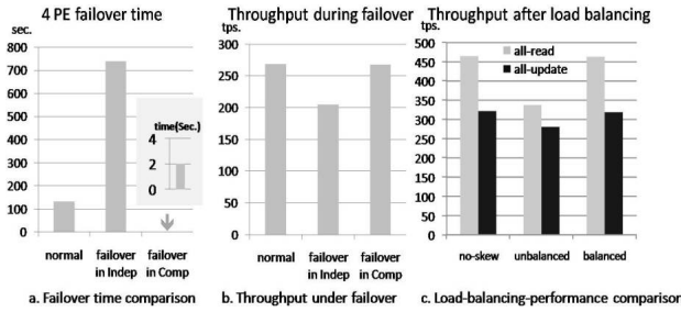
Fig. 14 Response time and failover and load-balancing performances.
