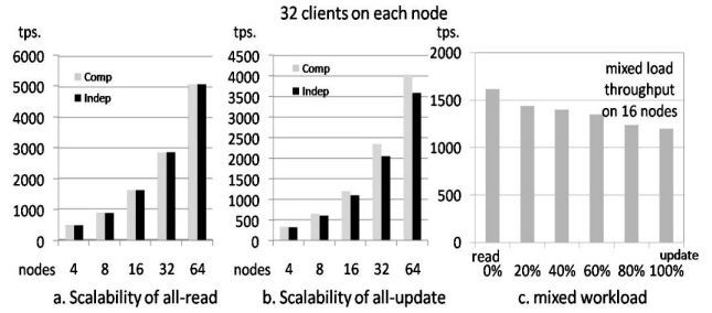
Fig. 11 Comparison of scalability.
