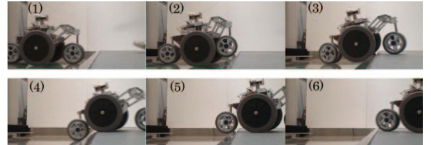
Fig. 18. Step climbing experiment: height of the step 80mm
