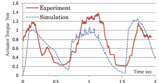
Fig. 20. Driving torque comparison between simulation and experiment negotiating 60mm height step
