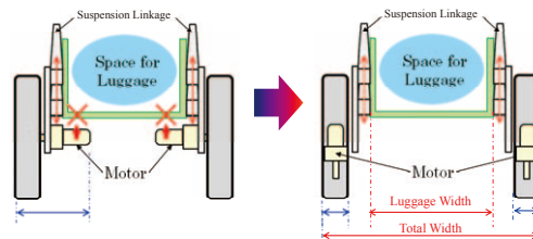
Fig. 10. Problem of the conventional actuator arrangement (left) and proposed arrangement (right)
