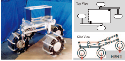
Fig. 3. Prototype model of the mars exploration rover “Hien II”
