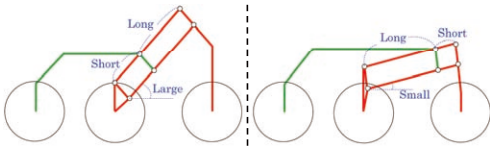
Fig. 6. Results of the static force analysis: suitable for front wheel negotiation (left), for rear wheel negotiation (right)
