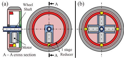
Fig. 11. Proposed low-profile in-wheel motor
