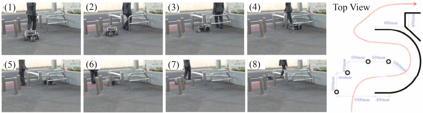
Fig. 21. An experiment passing through bollards in outdoor environment at 2.0sec interval capture (left), top view of the path (right)
