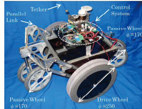
Fig. 14. Overview of the prototype
