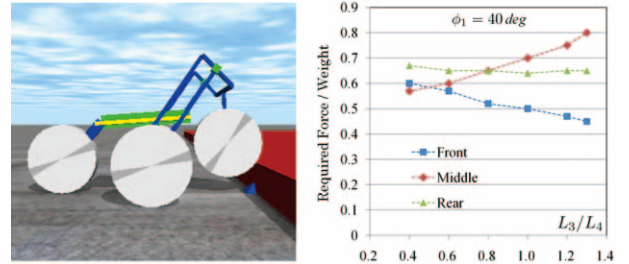
Fig. 8. An example of ODE simulation (left) and required force (right)
