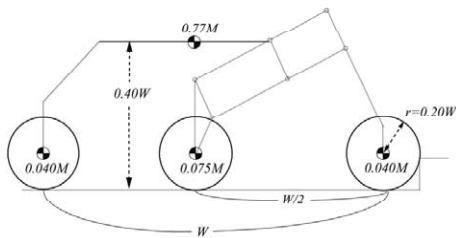
Fig. 7. Simulation model for the dynamics simulator
