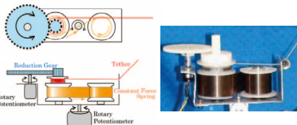
Fig. 13. Tether mechanism to measure the tether length and the direction
