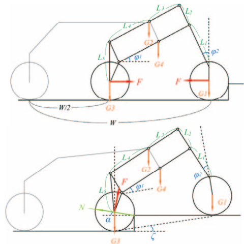
Fig. 5. Static force analysis: front wheel negotiating (top), middle wheel negotiating (bottom)
