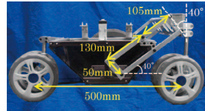
Fig. 9. Hardware implementation with the optimized link parameters (the middle wheel is not attached)
