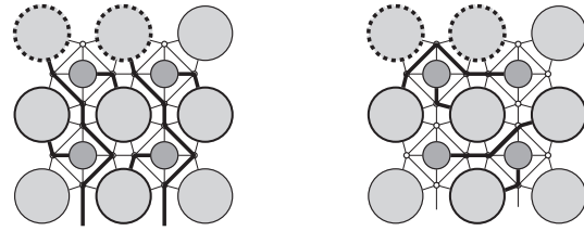
(a) Nearest via assignment. (b) Non nearest via assignment.
