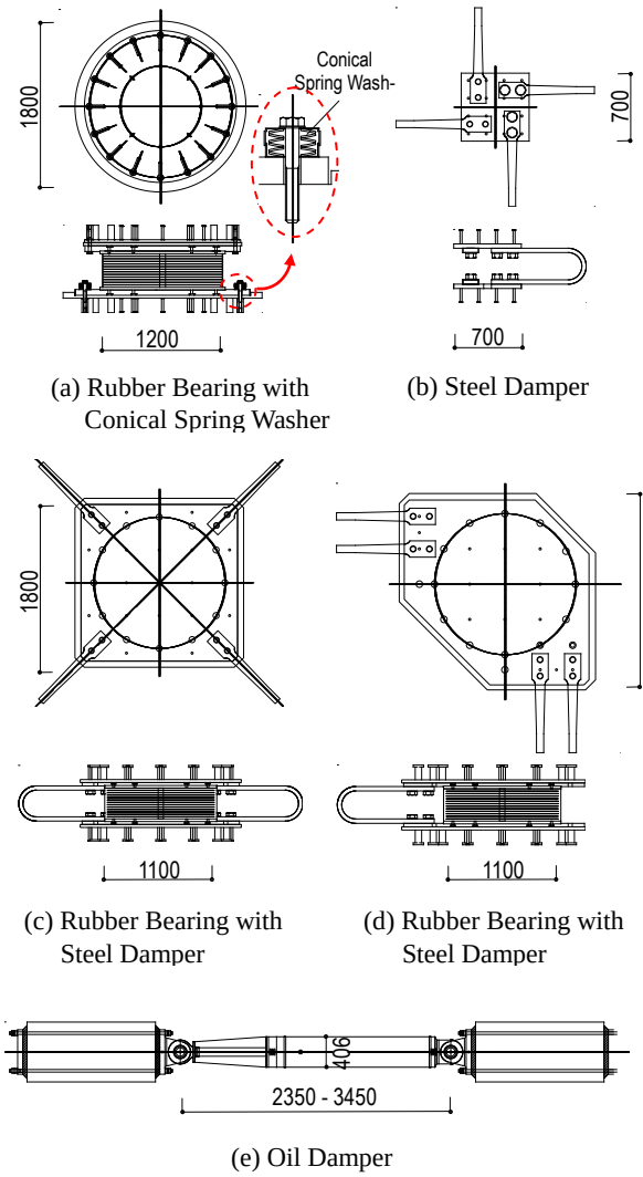
Figure 3. Rubber Bearing and Damper (unit: mm)
