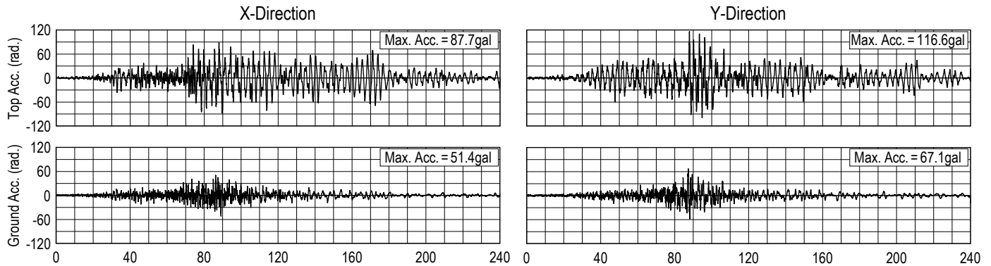
Figure 6. Acceleration time history
