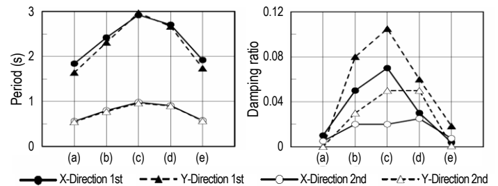
Figure 14. Vibration periods and damping ratios obtained before and after significant earthquake
