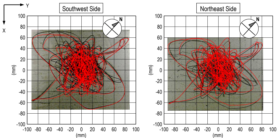
Figure 8. Trace recorder (black lines) vs. wire type displacement sensors (red lines).
