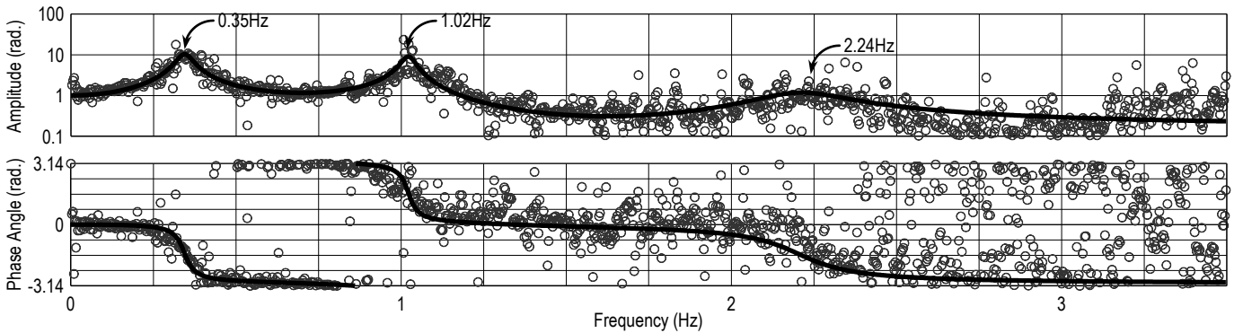
(a) Case 1: derived from records at 20th floor and 1st floor (below isolator)
