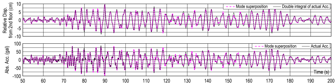
(b) Case 2: Analysis of superstructure only, using 2nd floor accelerations as input.
