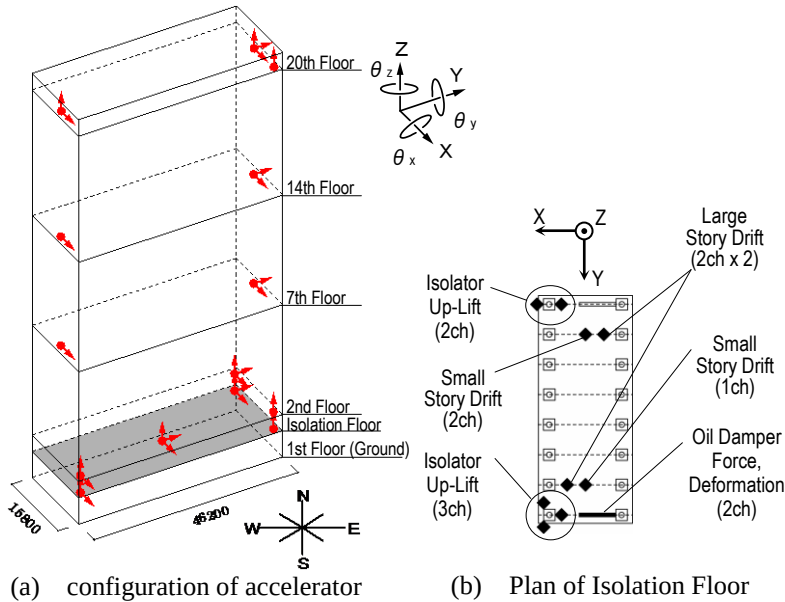
Figure 4 Monitoring System
