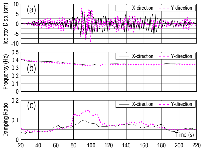
Figure 13. Variation of dynamic properties (a) isolation system displacements, (b) first mode natural frequencies and (c) first mode damping ratios
