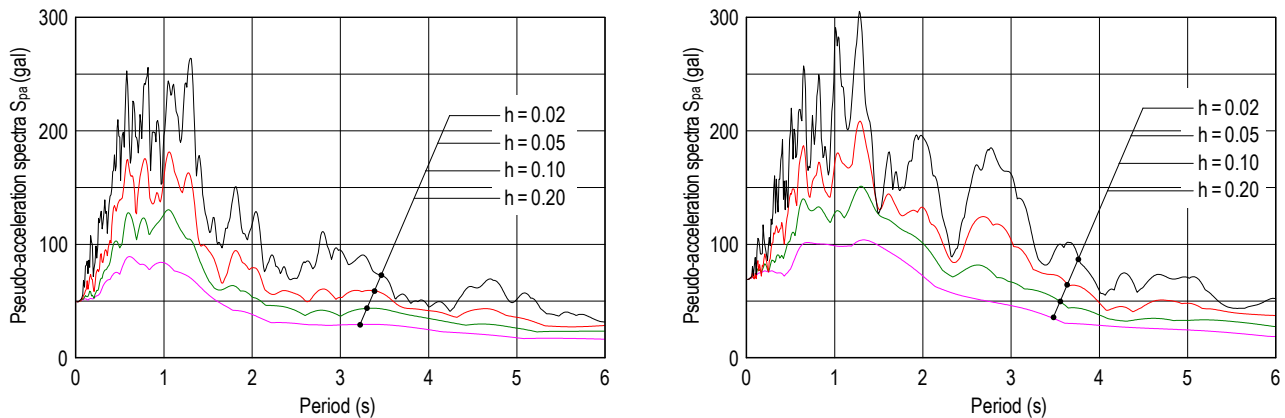
Figure 7. Response spectra for base motions in X and Y directions
