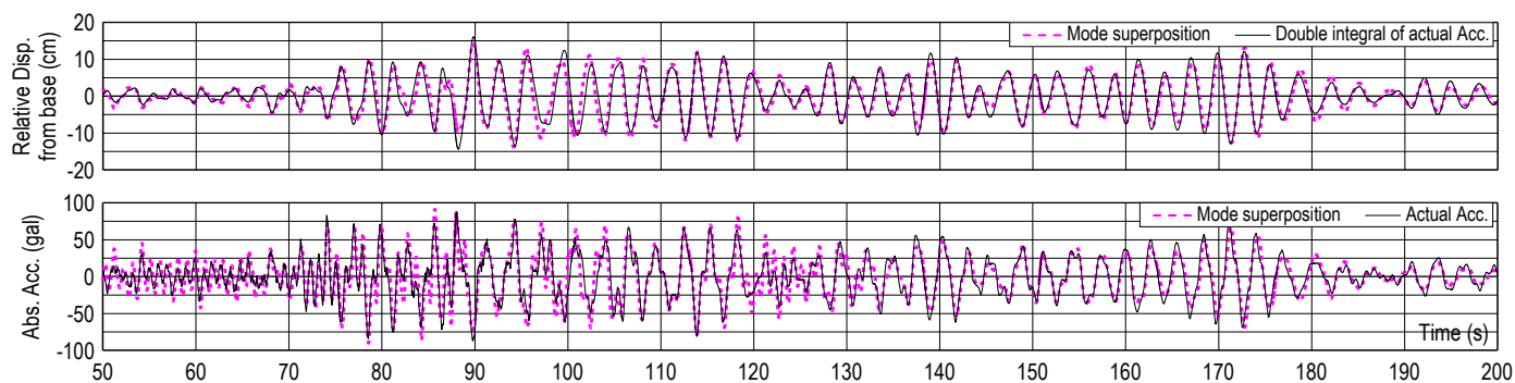
(a) Case 1: Analysis of whole structure (isolation system included), using 1st floor accelerations as input.
