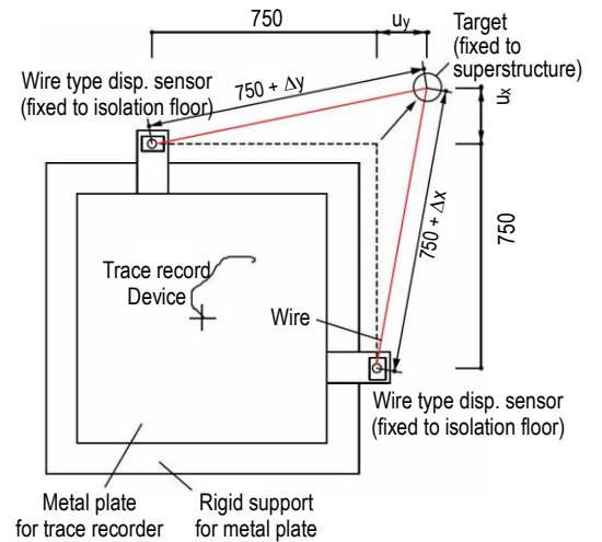
Figure 5. Measurement Device for Large Story Drift in Isolated Story (unit: mm)
