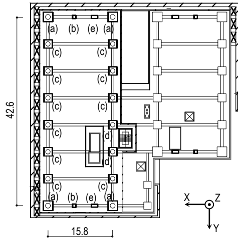
Figure 2 Seismic Isolation Floor (unit: m)
