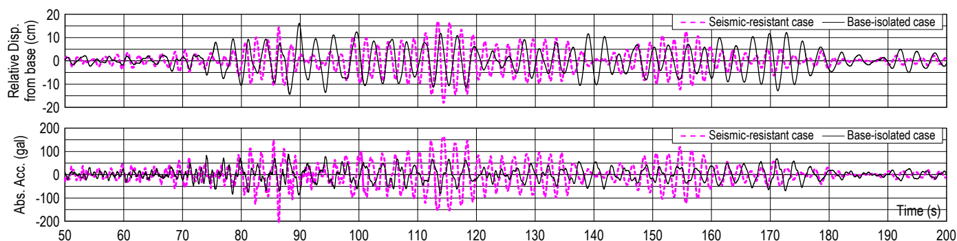
Figure 11. Comparison of base-isolated case and seismic-resistant case by modal analysis (Top of X-direction)
