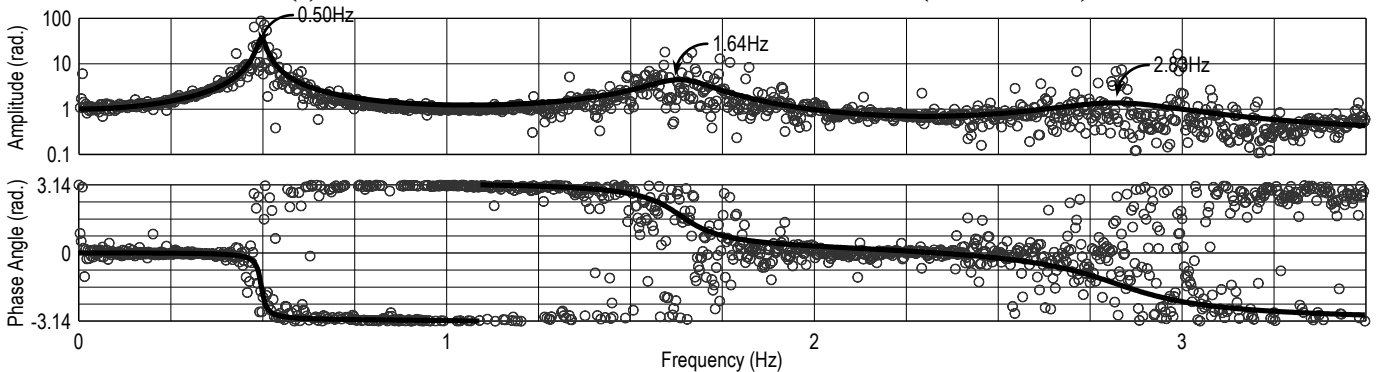
(b) Case 2: derived from records at 20th floor and 2nd floor (above isolator)
