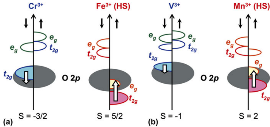
FIG. 8. Schematic band structures of (a) a \text{Cr}^{3+} – \text{Fe}^{3+} –O compound and (b) a \text{V}^{3+} – \text{Mn}^{3+} (HS)–O compound having antiferromagnetic spin ordering. Energy levels of empty bands are tentatively assigned.
