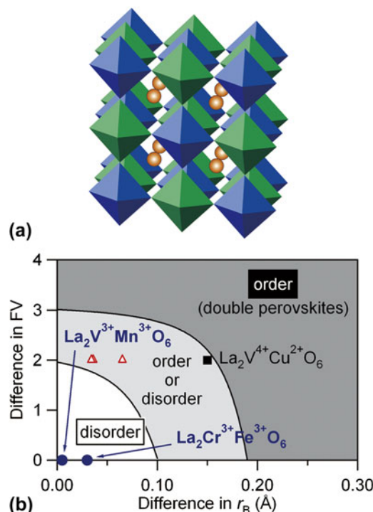
FIG. 1. (a) Schematic unit lattice of double perovskite \text{A}_2\text{B}'\text{B}''\text{O}_6 . The transition metals \text{B}' and \text{B}'' surrounded with six coordinated oxygen ions (represented by blue and green octahedral, respectively) form a rock-salt-type sublattice. (b) Bulk phase diagram as a function of differences in FV and ionic radii ( r_B ) (adopted from Ref. 2). The double perovskite oxides investigated in this study are marked by filled circles and square. Open triangles represent high T_C half-metallic ferrimagnets, \text{Sr}_2\text{B}'\text{B}''\text{O}_6 ( \text{B}'\text{B}'' = \text{CrRe}, \text{FeMo}, \text{FeRe} , from left to right in the figure).
