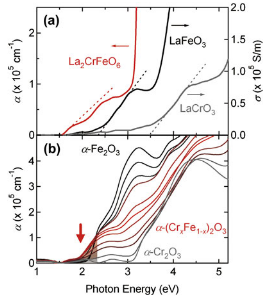
FIG. 7. (a) Optical absorption spectrum of LCFO film taken at room temperature and optical conductivity spectra of parent compounds, \text{LaCrO}_3 and \text{LaFeO}_3 bulks. 27 (b) Optical absorption spectra of \alpha-(\text{Cr}_x\text{Fe}_{1-x})_2\text{O}_3 films ( x = 0, 0.05, 0.15, 0.25, 0.4, 0.5, 0.6, 0.74, 0.85, 0.95 , and 1 ). 23 Arrow and shaded region indicate absorption band assignable to a transition from O 2p/\text{Cr } 3d(t_{2g}) to Fe 3d(t_{2g}) .
