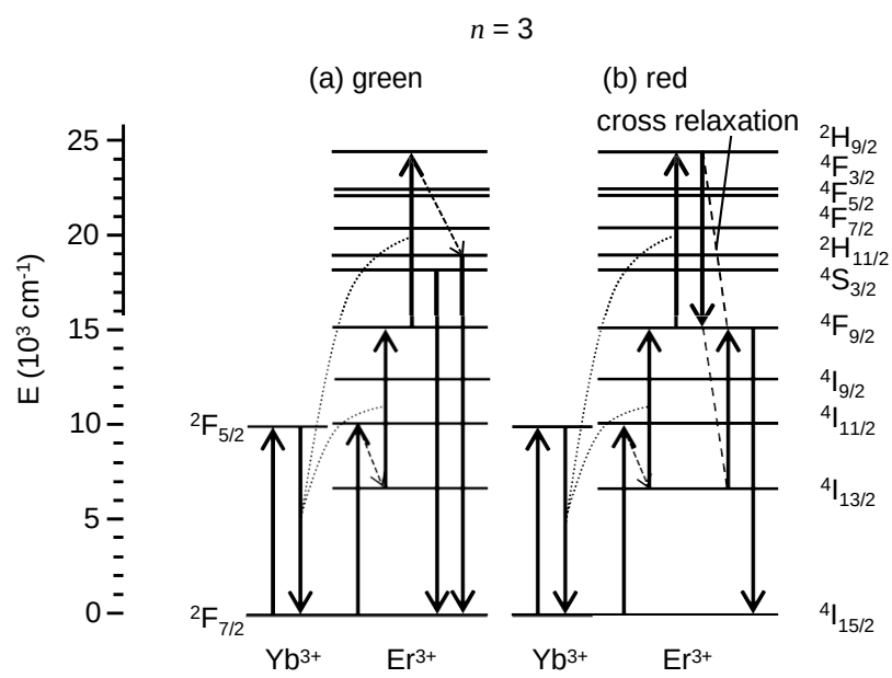
Figure 8. Three-photon processes in an energy diagram of an Er^{3+} ion: (a) green emission and (b) red emission.
