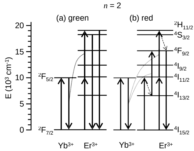
Figure 6. Two-photon processes in energy diagram of \text{Er}^{3+} ion: (a) green emission and (b) red emission.
