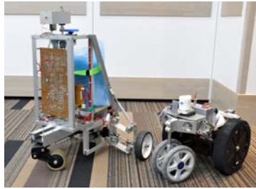
Fig. 2 Middle-sized prototype(left), small-sized prototype(right)
