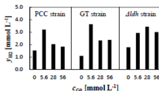
Figure 1: Hydrogen production per unit volume of cell suspension by PCC, GT and Aldh strain in buffer solutions containing 0, 5.6, 28 and 56 mmol L -1 of D-glucose at 96 h.
