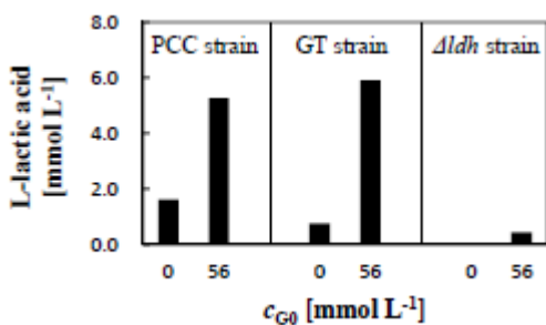
Figure 3: Concentration of L-lactic acid produced by PCC, GT and Aldh strain in buffer solutions containing 0 or 56 mmol L^{-1} of D-glucose at 96 h.
