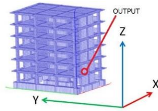
Figure 7: FE mesh.
