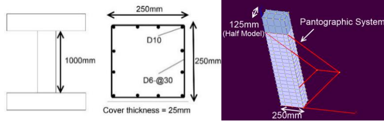
Figure 1: Design of the column.
