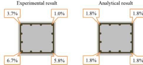
Figure 3: Comparison of average mass loss of reinforcing bars at each point.
