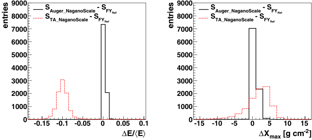
Figure 4. Left: difference of reconstructed primary energy of air showers. S_{\text{Auger\_NaganoScale}} - S_{\text{FYRef}} : mean 0.34%, RMS 1.22%; S_{\text{TA\_NaganoScale}} - S_{\text{FYRef}} : mean -9.98\% ; RMS 1.76%. Right: difference of reconstructed position of shower maximum of air showers. S_{\text{Auger\_NaganoScale}} - S_{\text{FYRef}} : mean 0.71 \text{ g cm}^{-2} , RMS 1.25 \text{ g cm}^{-2} ; S_{\text{TA\_NaganoScale}} - S_{\text{FYRef}} : mean 1.63 \text{ g cm}^{-2} ; RMS 3.56 \text{ g cm}^{-2} .
