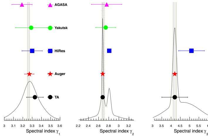
Figure 3. Spectral indices for the triple-power law fits from Table 1. The solid black line is the sum of the Gaussian probability distributions implied by the errors in the indices. The shaded bar represents the weighted mean of the measurements and its uncertainty.
