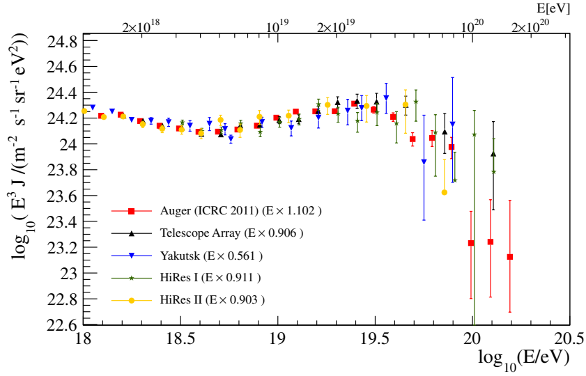
Figure 6. Re-scaled spectra from Figure 5, but in the form E^3 J .
