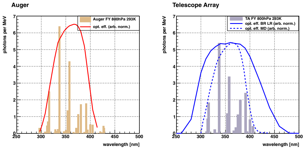
Figure 8. Optical efficiency curves (arbitrary normalization) together with the assumed fluorescence spectra for Auger and the Telescope Array. The spectra are for dry air at a pressure of 800 hPa and a temperature of 293 K. In the case of the Telescope Array, there are different optical efficiency curves for the Black Rock and Long Ridge sites on one hand, and the former HiRes telescopes now at the Middle Drum site on the other.
