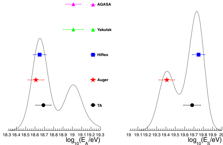
Figure 4. Break-point energies for the triple-power law fits from Table 1. The solid black line is the sum of the Gaussian probability distributions implied by the errors in the break-point energies. Those errors are the statistical uncertainty folded with the systematic uncertainty in the energy scale.
