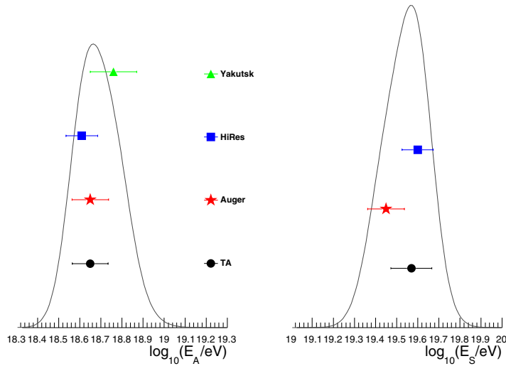
Figure 7. Break-point energies for the triple-power law fits after energy rescaling, to be compared with the original positions in Figure 4. The error bars again represent the statistical uncertainty folded with the systematic uncertainty in the energy scale for each experiment. The reference spectrum is the average of Auger and TA.
