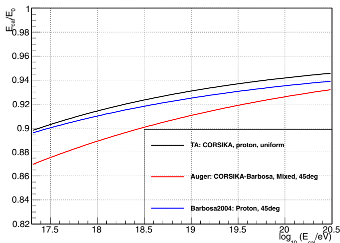
Figure 9. Comparison of the conversion factors from calorimetric energies to primary energies. See text for details.
