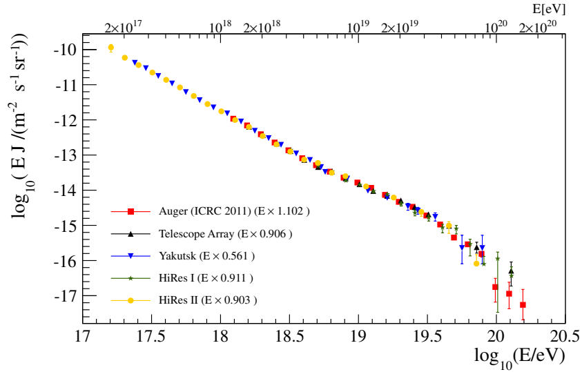
Figure 5. Spectra from Figure 2 after energy-rescaling. The reference spectrum is the average of those from Auger and TA. The values of \log_{10} \alpha are given in Table 3, and the values of \alpha are indicated on the plot.
