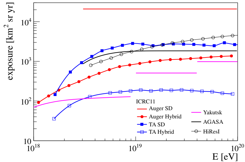
Figure 1. Exposures of the experiments at the time of the ICRC 2011 conference for Auger SD [1], Auger Hybrid [1], TA SD [2], TA Hybrid [3], Yakutsk SD [4], AGASA [5] and HiRes I [6]. After M. Unger [7].
