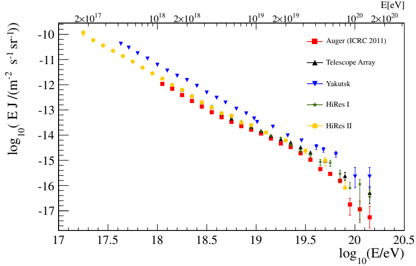
Figure 2. Published energy spectra, with the flux multiplied by E , for Auger (combined Hybrid/SD) [1], TA SD [2], Yakutsk SD [4], HiRes I [8], and HiRes II [8].
