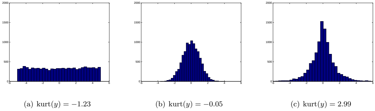
Figure 2.7: Kurtosis
