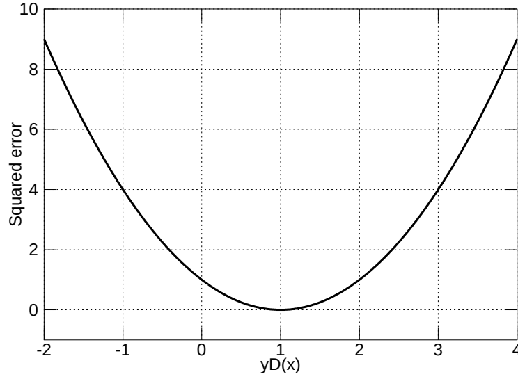
Figure 4.10: Squared error
