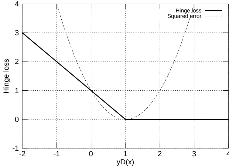
Figure 4.17: Hinge loss
