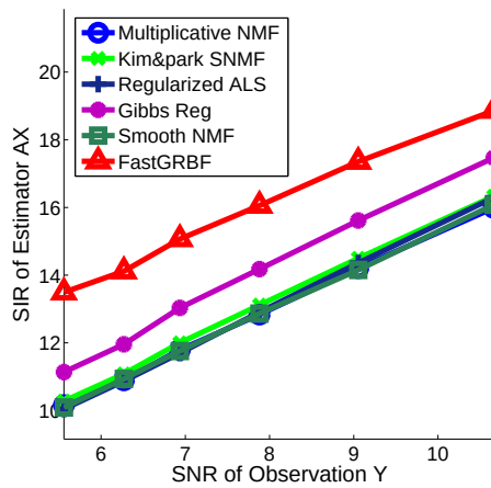
(e) Evaluation with SIR of \mathbf{AX}
