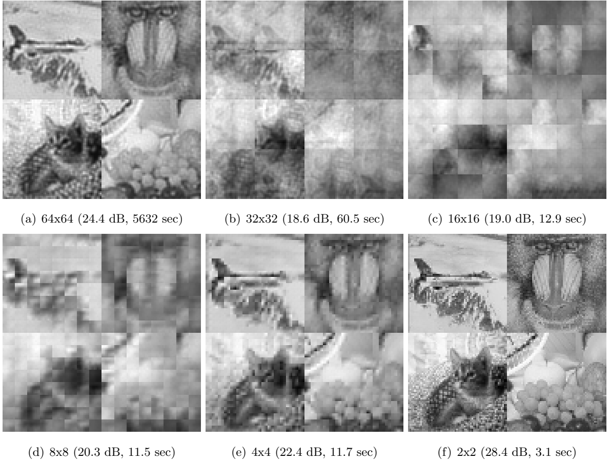
Figure 7.9: Results of fastGRBF-block-NMF
