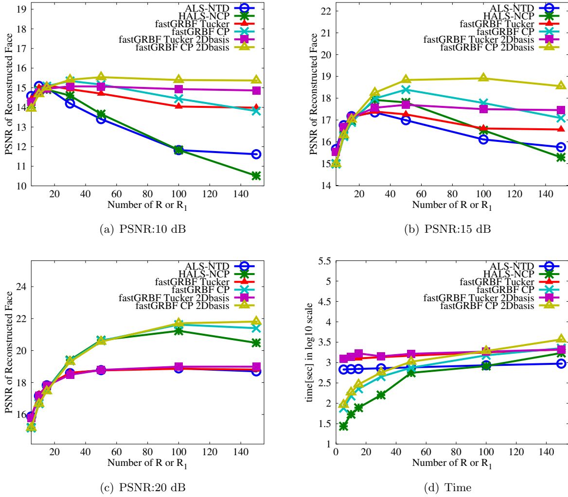
Figure 7.4: PSNR of NTF results on 165 (11×15) faces for various ranks
