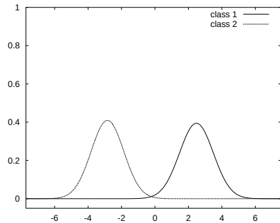
(e) KFDA
