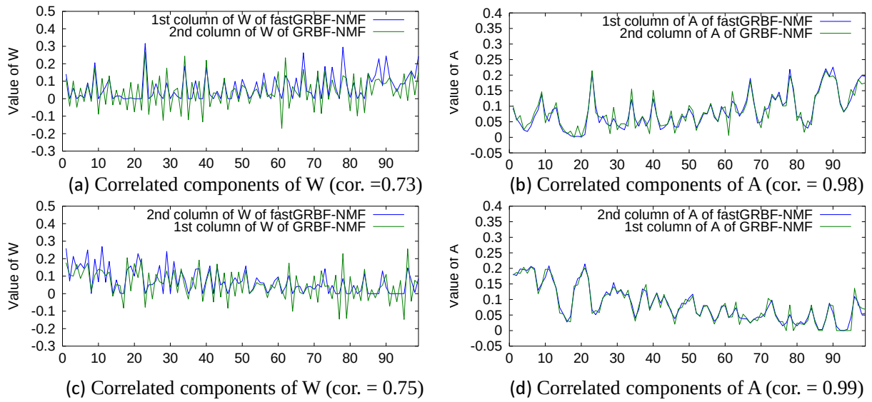
Figure 7.2: Values of \mathbf{W} and \mathbf{A} obtained by the fastGRBF-NMF and the GRBF-NMF
