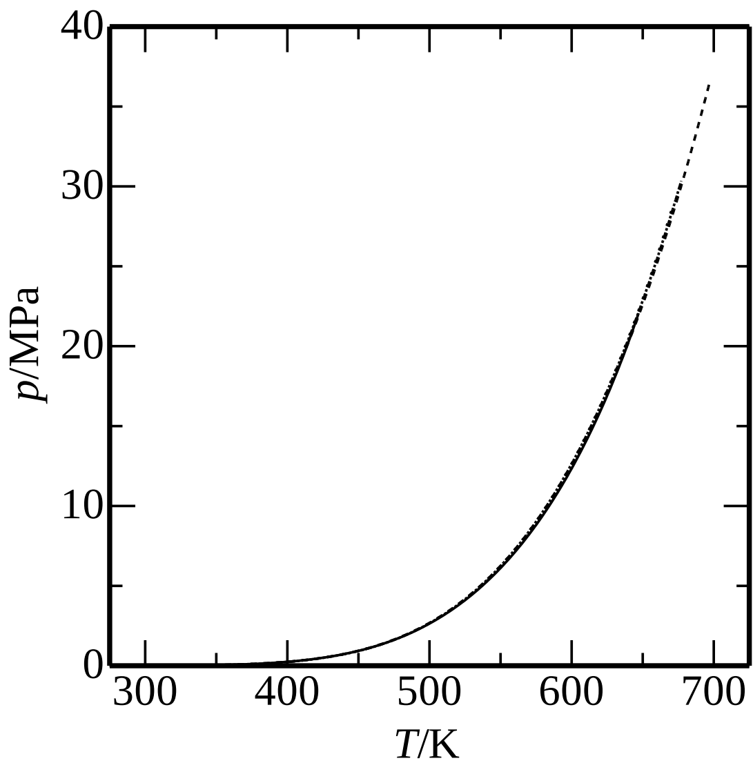
Fig. 5.7 Vapor pressure for water; calculated with (---), 2-site model; (···), 3-site model, (-·-), 4-site model; (—), experimental data [40].
