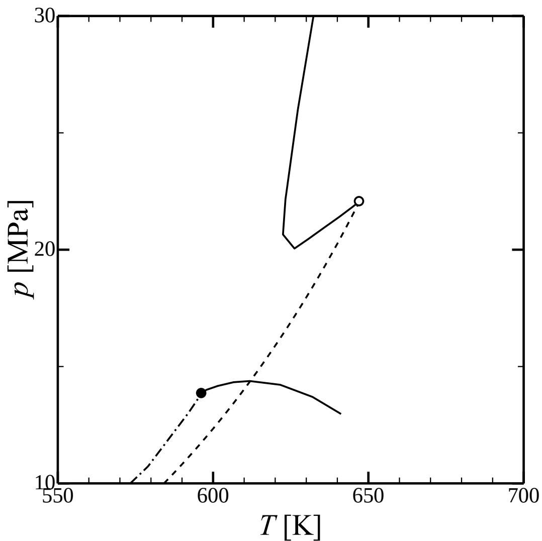
Fig. 1.9 p - T projection for decalin + water binary system [7]; (-·-), vapor-liquid-liquid three phase line; (—), vapor-liquid and liquid-liquid critical curve; (---), vapor pressure; (○), critical point; (●), upper critical end point.
