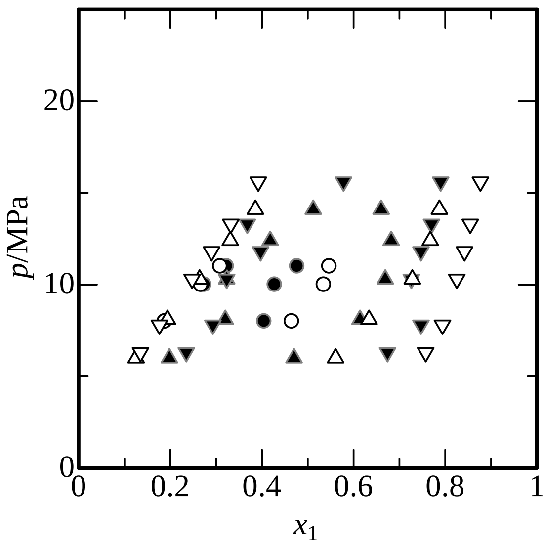
Fig. 6.6 Phase equilibria for water (1) + 1-methylnaphthalene (2) + p -xylene (3) ternary system at 653 K and z = (\circ) , 0.25; ( \triangle ), 0.50; ( \nabla ), 0.75 for calculated; z = (\bullet) , 0.25; ( \blacktriangle ), 0.50; ( \blacktriangledown ), 0.75 for experimental.
