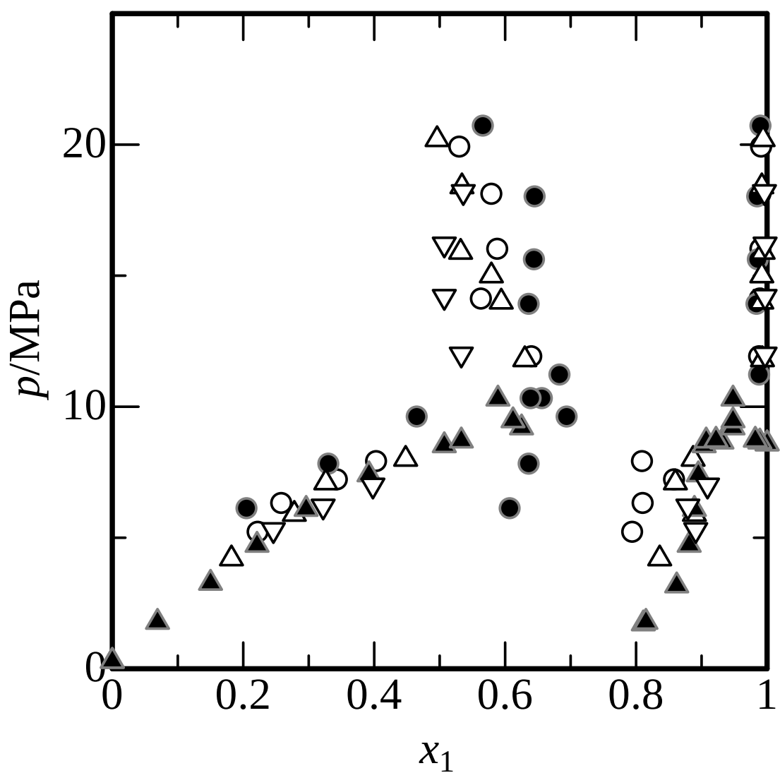
Fig. 3.1 Phase equilibria for water (1) + 1-methylnaphthalene (2) + p -xylene (3) ternary system at 573 K; z = (\bigcirc) , 0.25; ( \triangle ), 0.50; ( \nabla ), 0.75. Binary systems for ( \blacktriangle ), water (1) + 1-methylnaphthalene (2) [24]; ( \bullet ), water (1) + p -xylene (3) in this work.
