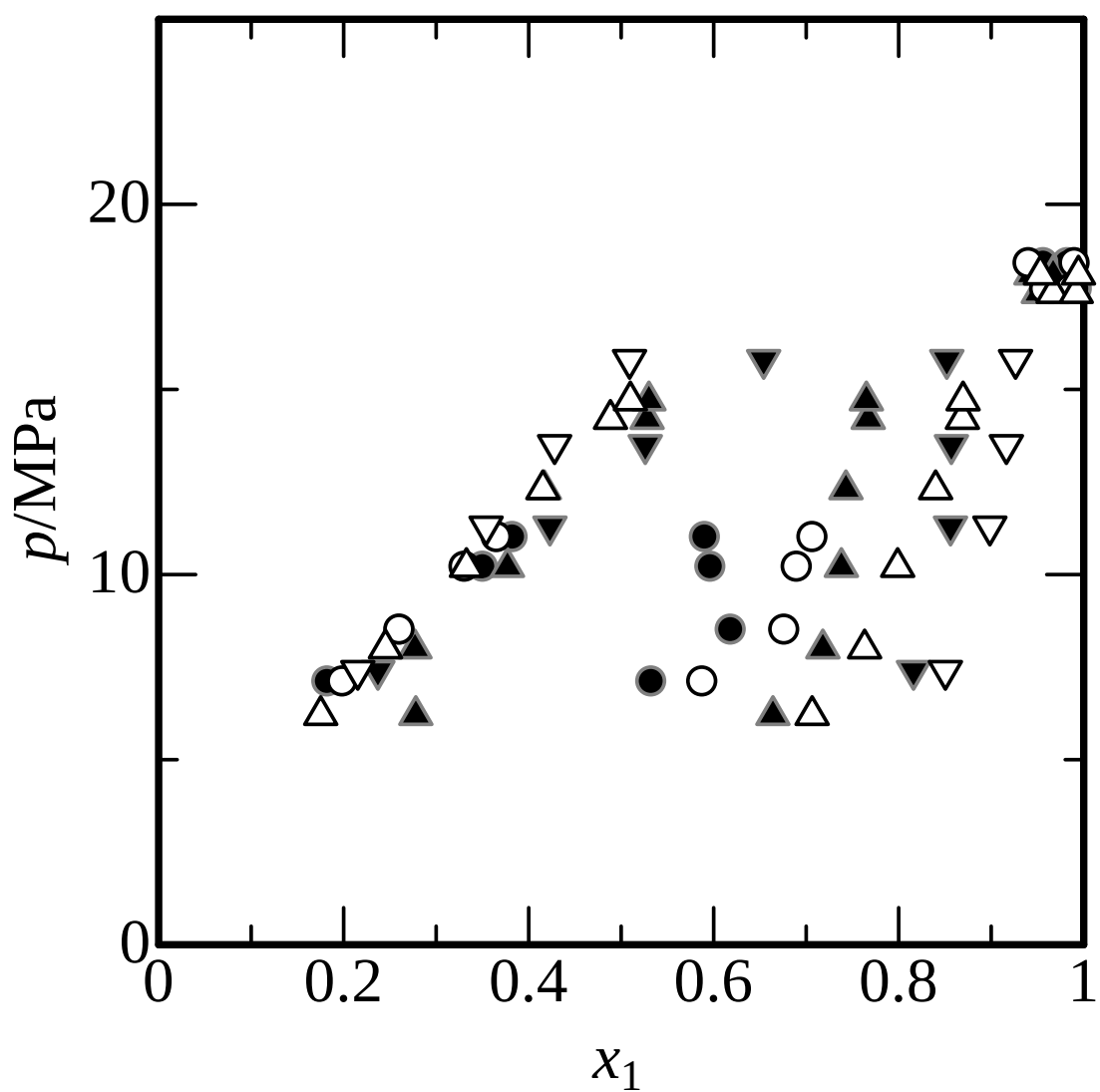
Fig. 6.5 Phase equilibria for water (1) + 1-methylnaphthalene (2) + p -xylene (3) ternary system at 623 K and z = (\bigcirc) , 0.25; (\triangle) , 0.50; (\nabla) , 0.75 for calculated; z = (\bullet) , 0.25; (\blacktriangle) , 0.50; (\blacktriangledown) , 0.75 for experimental.
