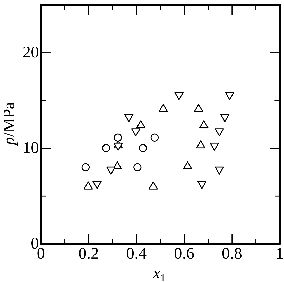
Fig. 3.4 Phase equilibria for water (1) + 1-methylnaphthalene (2) + p -xylene (3) ternary system at 653 K; z = (\bigcirc) , 0.25; ( \triangle ), 0.50; ( \nabla ), 0.75.
