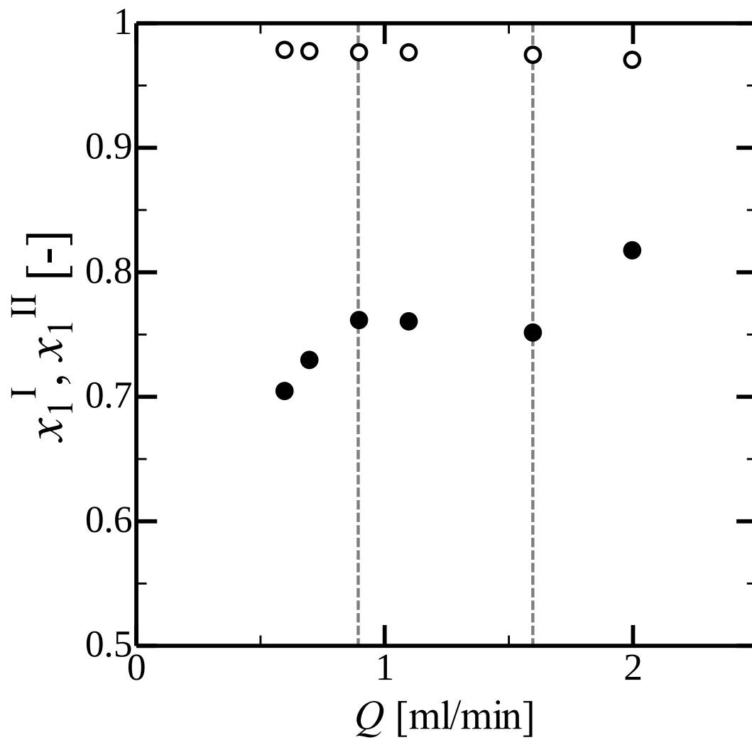
Fig. 2.7 Flow rate dependence on liquid-liquid equilibrium data at 583 K and 15.2 MPa; ( \bullet ), hydrocarbon rich phase; ( \circ ), water rich phase.
