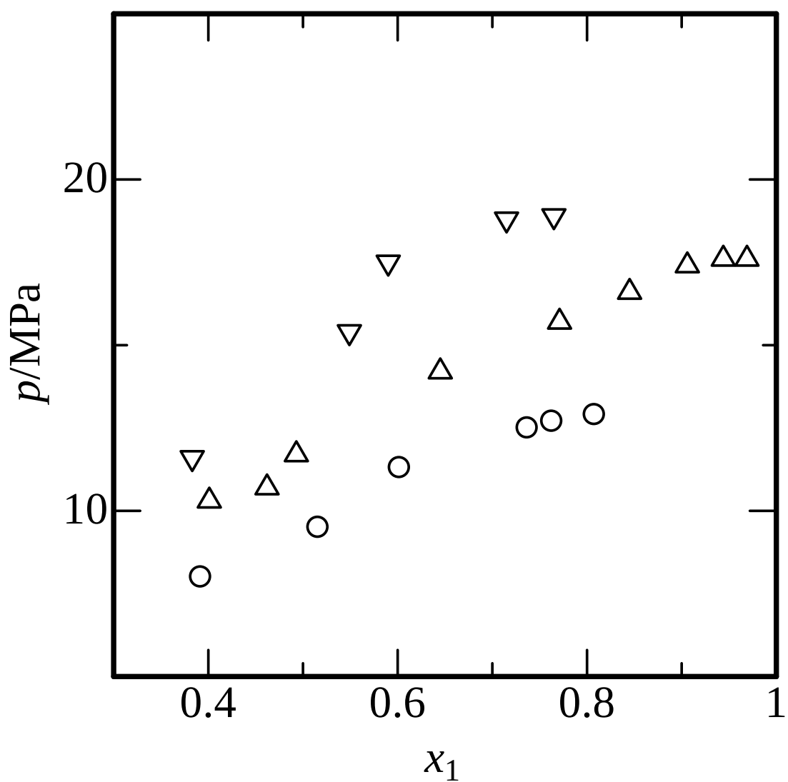
Fig. 3.5 Phase equilibria for water (1) + squalane (2) + 1-methylnaphthalene (3) ternary system for z = 0.01 at ( \bigcirc ), 603 K; ( \triangle ), 623 K; ( \nabla ), 653 K.
