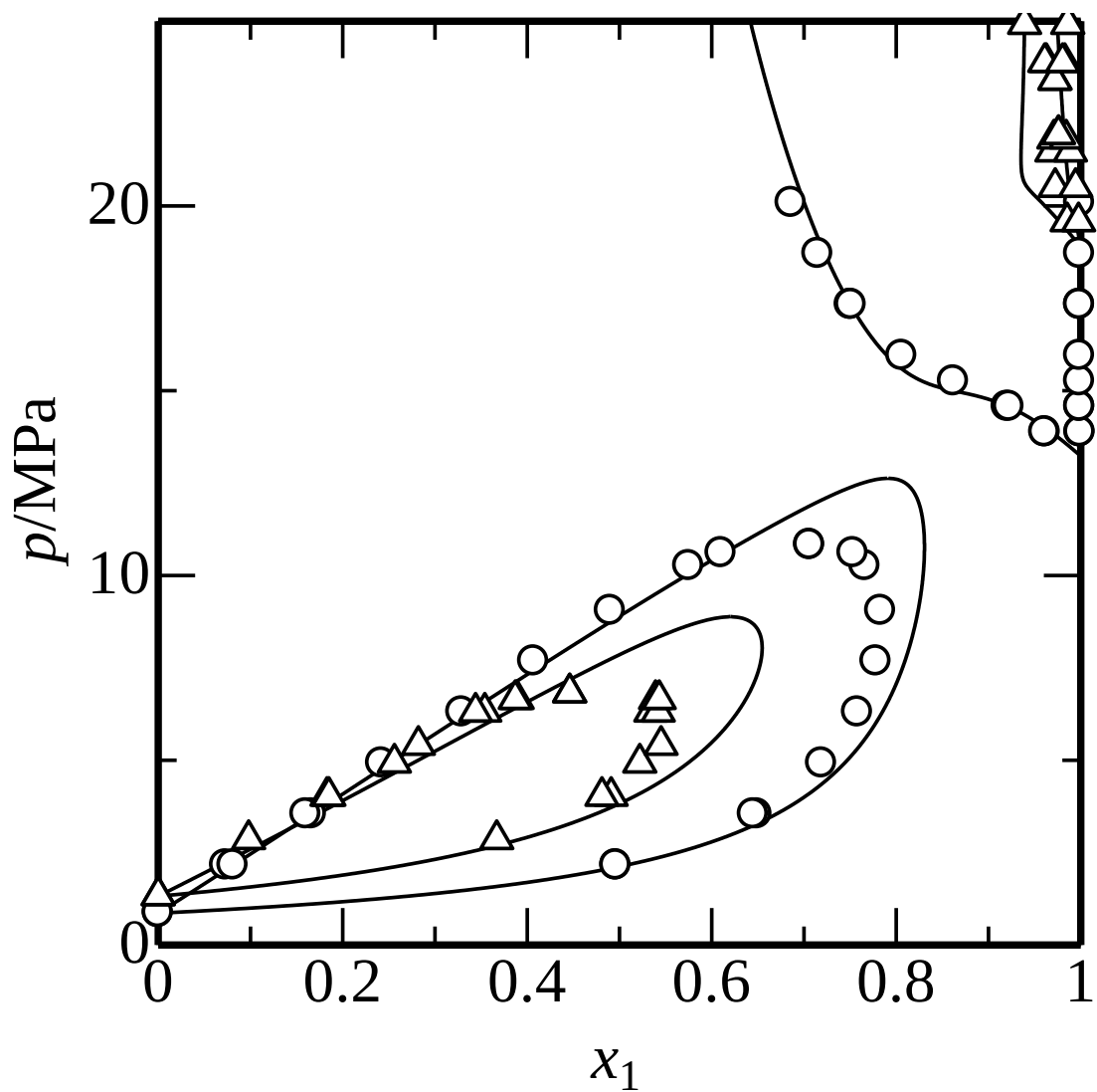
Fig. 5.10 Phase equilibria for water (1) + dodecane (2) system at (○), 604 K; (Δ), 633 K [25]. (—), calculated.
