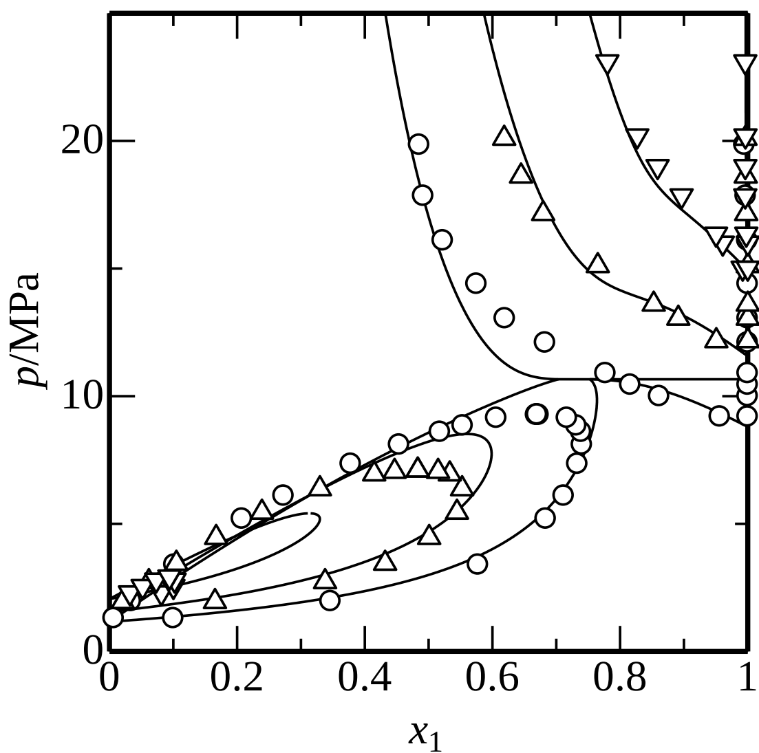
Fig. 5.9 Phase equilibria for water (1) + decane (2) system at ( \circ ), 573 K; ( \Delta ), 593 K; ( \nabla ), 613 K [41]. (—), calculated.
