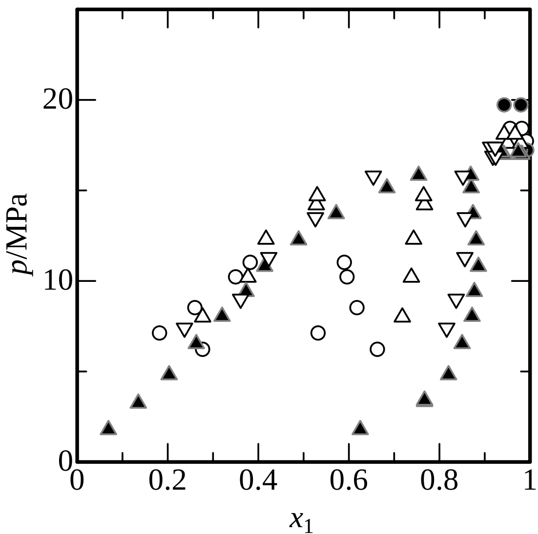
Fig. 3.3 Phase equilibria for water (1) + 1-methylnaphthalene (2) + p -xylene (3) ternary system at 623 K; z = (\bigcirc) , 0.25; (\triangle) , 0.50; (\nabla) , 0.75. Binary systems for (\blacktriangle) , water (1) + 1-methylnaphthalene (2) [24]; (\bullet) , water (1) + p -xylene (3) in this work.
