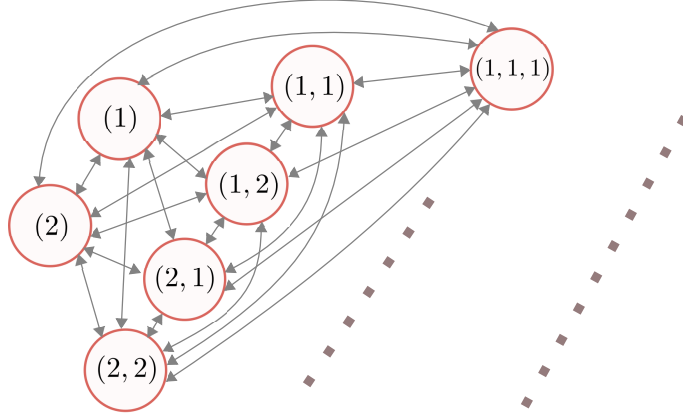
Figure 9.3: Transition diagram of the sequence-valued discrete-time countable-state Markov chain \{s(i) \in \mathcal{S} \triangleq \{(1), (2), (1, 1), \dots\}_{i \in \mathbb{N}_0}\} over the set of mode sequences of variable length
