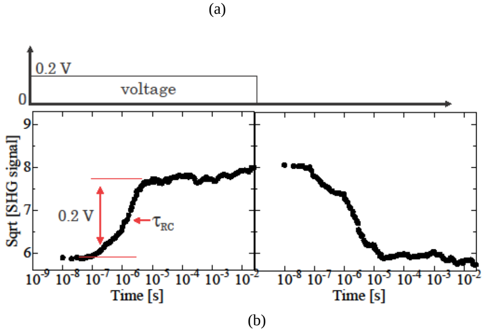
Figure 3.7: EFISHG measurements under square-wave voltage application ( V_{ex} \sim V_{oc} ).
