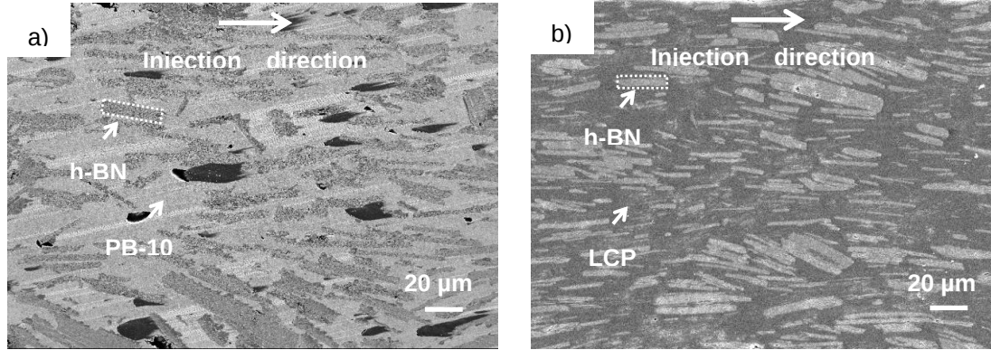
Figure 6. SEM images of the cross-sectional surface (ND, MD) for the a) molded PB-10-I composite (30 vol%) and b) molded LCP composite (29 vol%). Scale bar, 20 \mu\text{m} .
