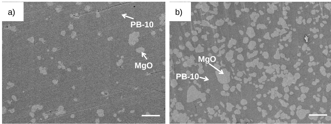
Figure 4. SEM images of the polished surface for PB-10 composites. a) 9 vol% and b) 29 vol%. Scale bar, 100 \mu\text{m} .
