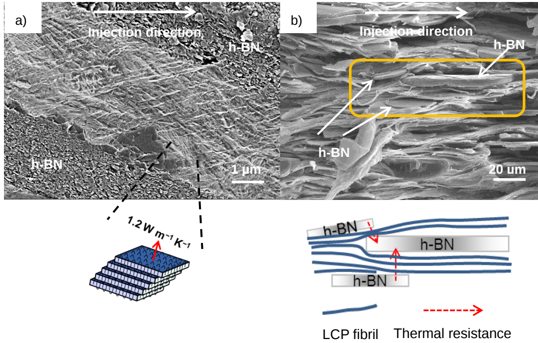
Figure 9. SEM images and schematic illustrations of the polymeric morphology between the h-BN platelets arranged one above the other. a) Molded PB-10-I composite (30 vol%). Scale bar, 1 μm. b) Molded LCP composite (29 vol%). Scale bar, 20 μm.
