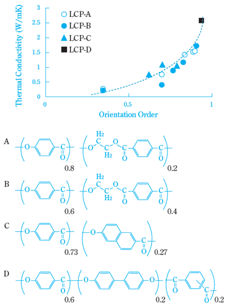
Figure 7. Relationship between orientation order of various LCP and thermal conductivity (reprinted from Ref. [20]).
