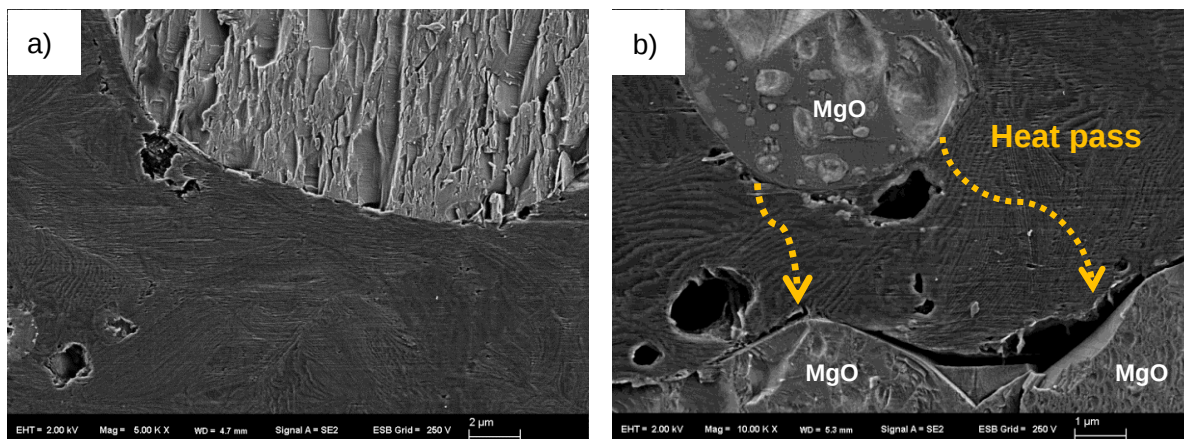
Figure 7. SEM images of a compression-molded PB-10/MgO composite at 9 vol% loading. a) A large gap between the MgO particles. Scale bar, 2 \mu\text{m} . b) A small gap between the MgO particles. Scale bar, 1 \mu\text{m} .
