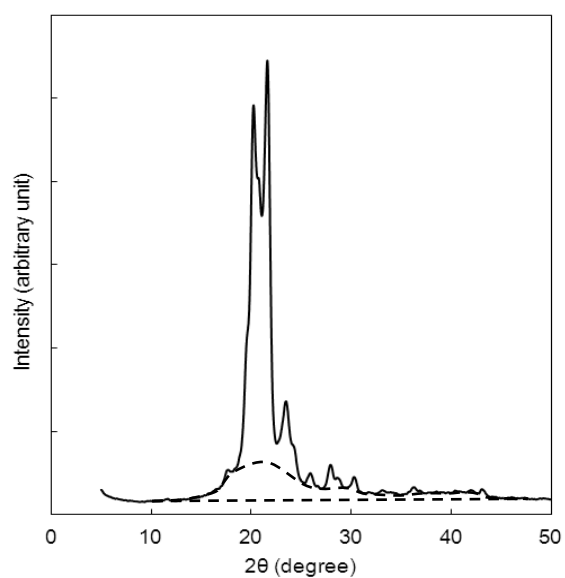
Figure 18. Powder XRD intensity profile of injection-molded PB-12, indicating the crystallinity of 70 to 80 %.
