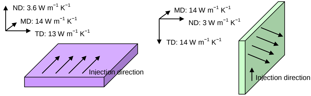
Figure 27. TC of base plate and fin part in a heat sink made of a composite A (14 W m -1 K -1 ).
