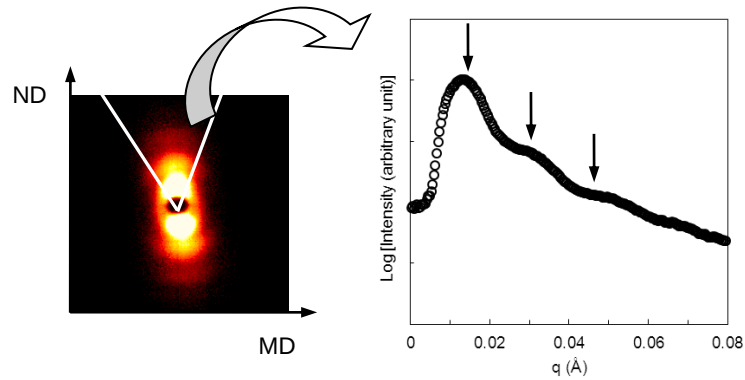
Figure 16. SAXS intensity profile of injection-molded PB-12 from the (ND, MD) pattern, indicating the lamellae with 41-nm thickness.
