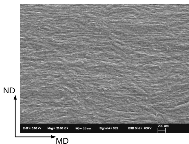
Figure 15. SEM image of PB-18 which is observed on a cross-sectional surface of (ND, MD) near the molding surface. Scale bar, 200 nm.
