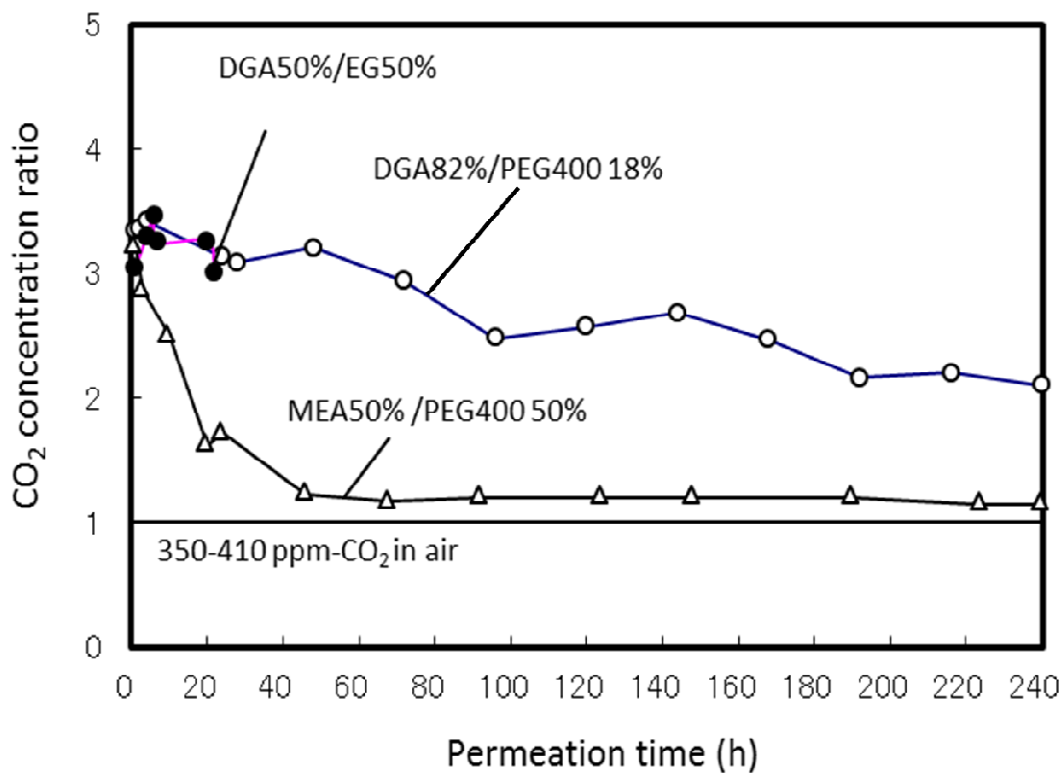
Fig. 2.6 Durability of the liquid membranes ( \delta = 19 \mu\text{m} , p_1 = 15 \text{ cmHg} , F_p = 1 \text{ L min}^{-1} , T = 297.15 to 299.15 \text{ K} ).
