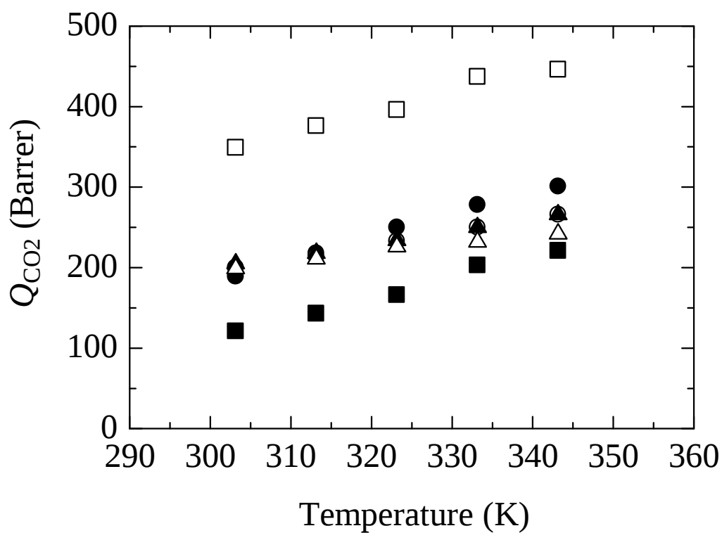
Fig. 3.6 Plot of CO 2 permeability against temperature through ionic liquid membranes, (●) [emim][BF 4 ], (○) [bmim][BF 4 ], (■) [bmim][PF 6 ], (□) [bmim][Tf 2 N], (▲) [bmim][OTf], (△) [bmim][dca].
