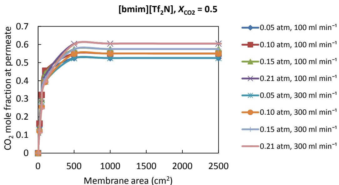
Fig. 6.5 Optimization of membrane area for CO 2 separation from CO 2 /N 2 mixed gas, (a) [bmim][PF 6 ] membrane at X_{CO_2} = 0.3 , (b) [bmim][Tf 2 N] membrane at X_{CO_2} = 0.3 , (c) [bmim][PF 6 ] membrane at X_{CO_2} = 0.4 , (d) [bmim][Tf 2 N] membrane at X_{CO_2} = 0.4 , (e) [bmim][PF 6 ] membrane at X_{CO_2} = 0.5 , (f) [bmim][Tf 2 N] membrane at X_{CO_2} = 0.5
