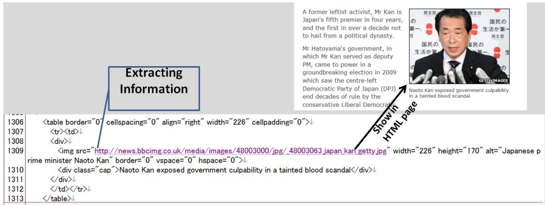
Figure 3.5: Object Extraction - Example
