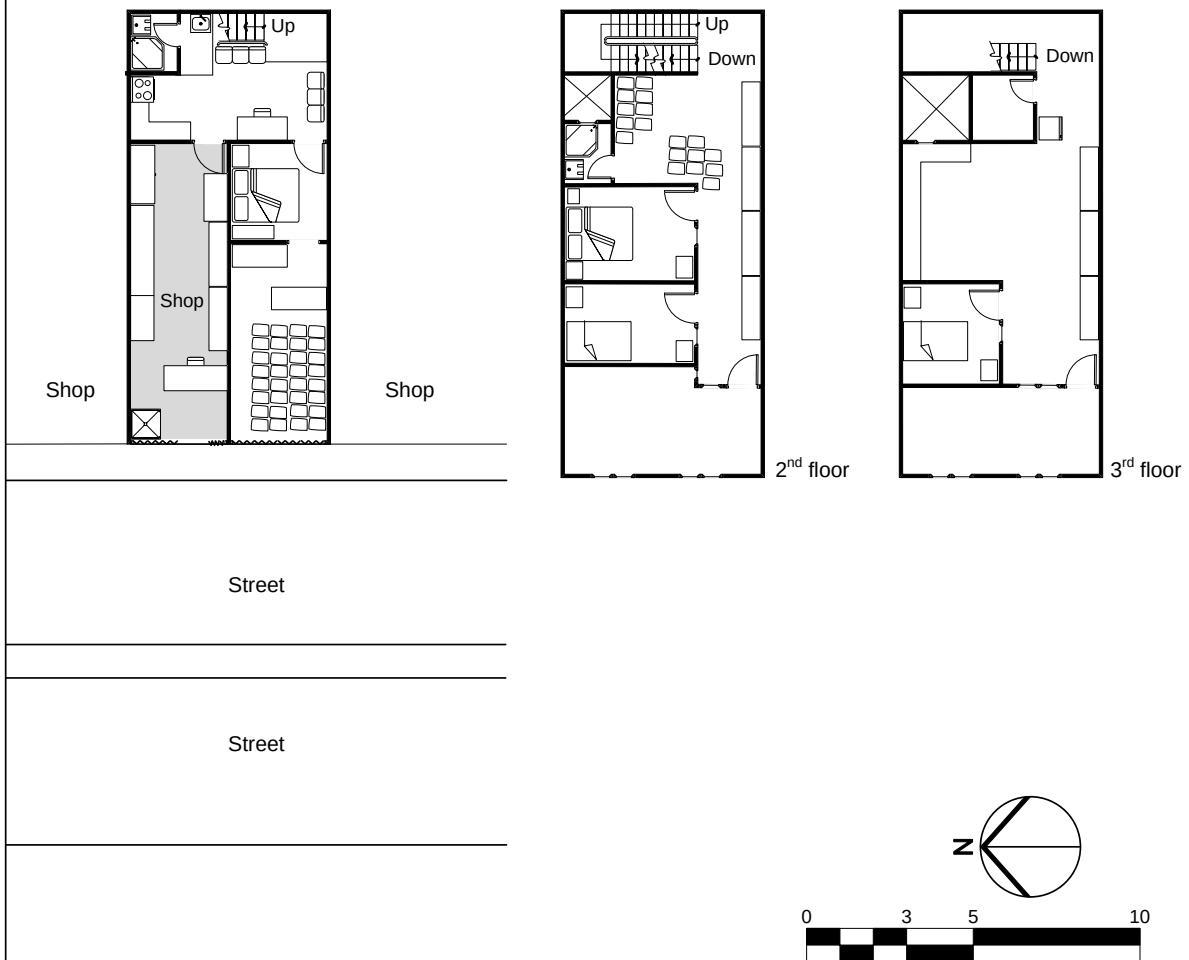
Floor Plan of the Chinese Shop House (C-06)
