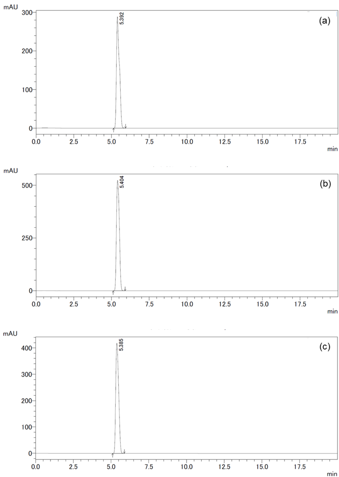
Figure 4-12: HPLC measurements of 8-A after (a) 32 hours, (b) 64 hours and (c) 144 hours of photoradiation in the solid state.
