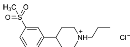
Scheme 1-9: Molecular structure of pridopidine hydrochloride.
