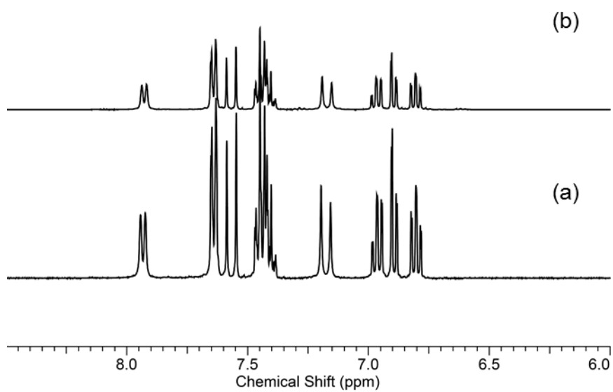
Figure 4-4: ^1\text{H} NMR results (a) before and (b) after thermal transformation.
