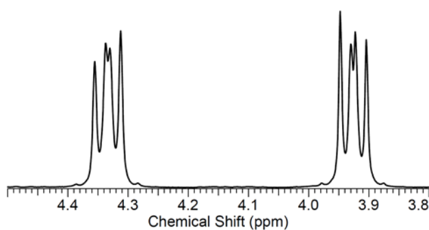
Figure 2-10: ^1\text{H} NMR spectra of 1 after irradiation for 5 hours in \text{DMSO}-d_6 . The signals are originated from the cyclobutane protons.
