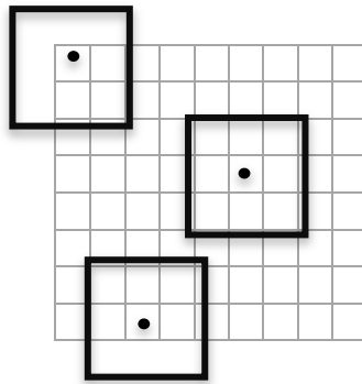
Fig. 3.2. 3 X 3 neighborhood blocks in a matrix
