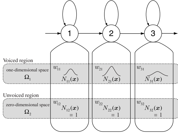
Figure 2.2: MSD-HMM [1].
