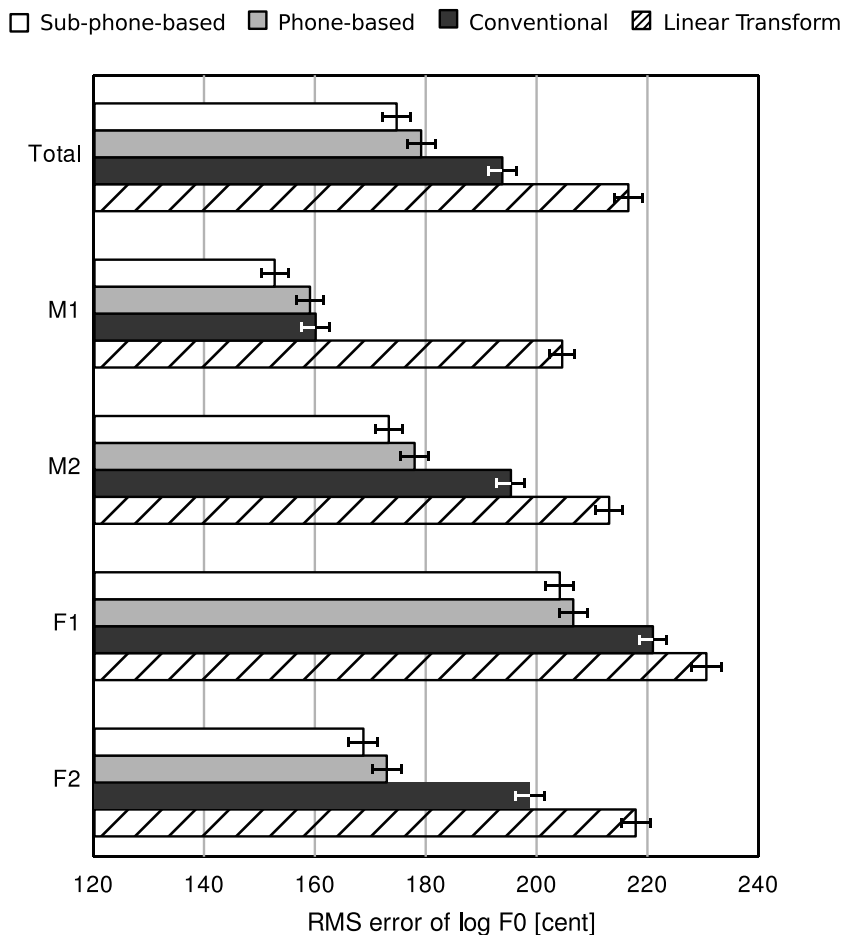
Figure 3.11: Comparison of average log F0 RMS errors.
