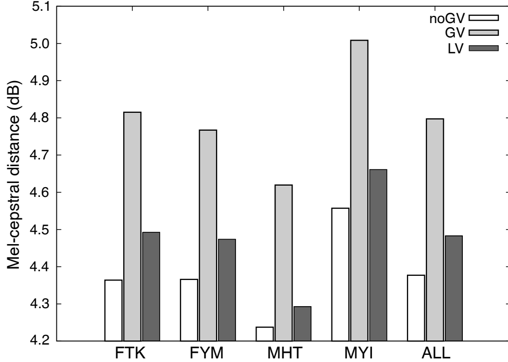
Figure 4.7: Average mel-cepstral distances between the original and synthetic speech.
