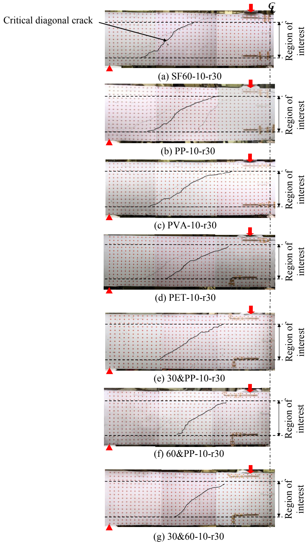
Figure 5.11 Critical diagonal crack at peak load of specimens in Series III
