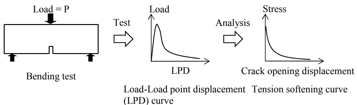
Figure 3.1 Tension softening curve analyzed from bending test
