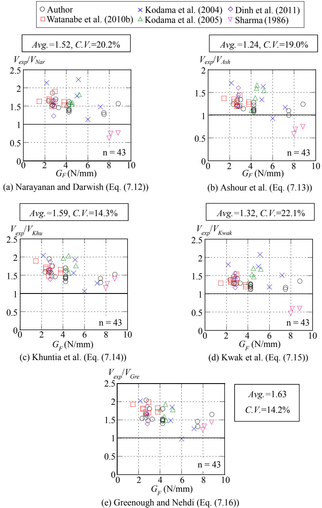
Figure 7.7 Accuracy of the equations proposed by other researchers
