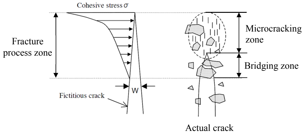
Figure 3.5 Fracture process zone (JCI-S-001-2003, 2003a)
