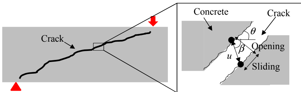
Figure 4.10 Definition of crack surface displacement ( u )
