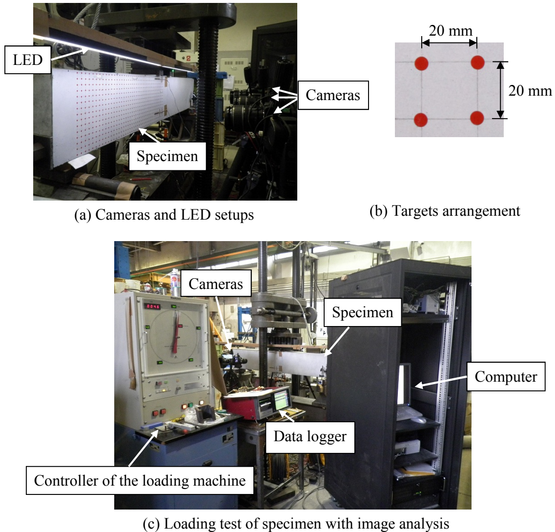
Figure 4.9 Preparation for the image analysis
