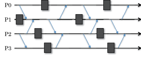
FIGURE 2.11: Uncoordinated checkpointing: message logging is required to ensure the checkpoints are consistent
