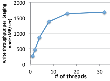
FIGURE 3.12: Impact of varying data writer count
