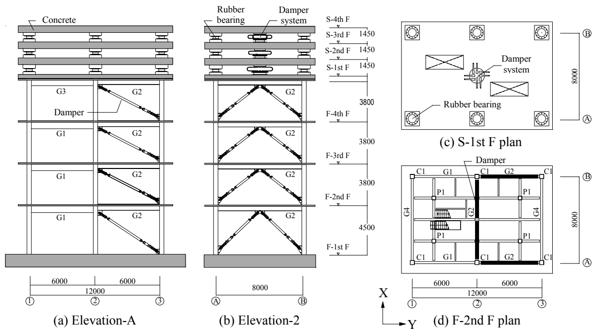
Figure 1. Plan and elevation of specimen (unit : mm)
