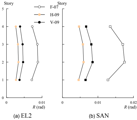
Figure 5. Maximum inter-story drift angle
