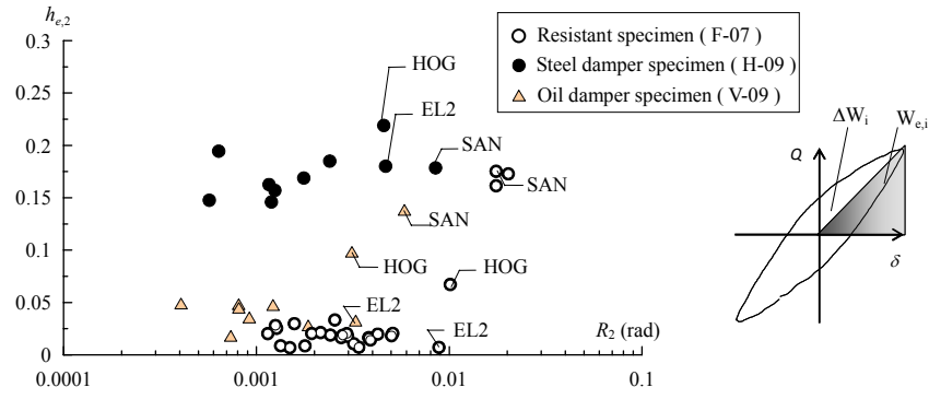
Figure 9. Equivalent damping ratio of 2 nd story
