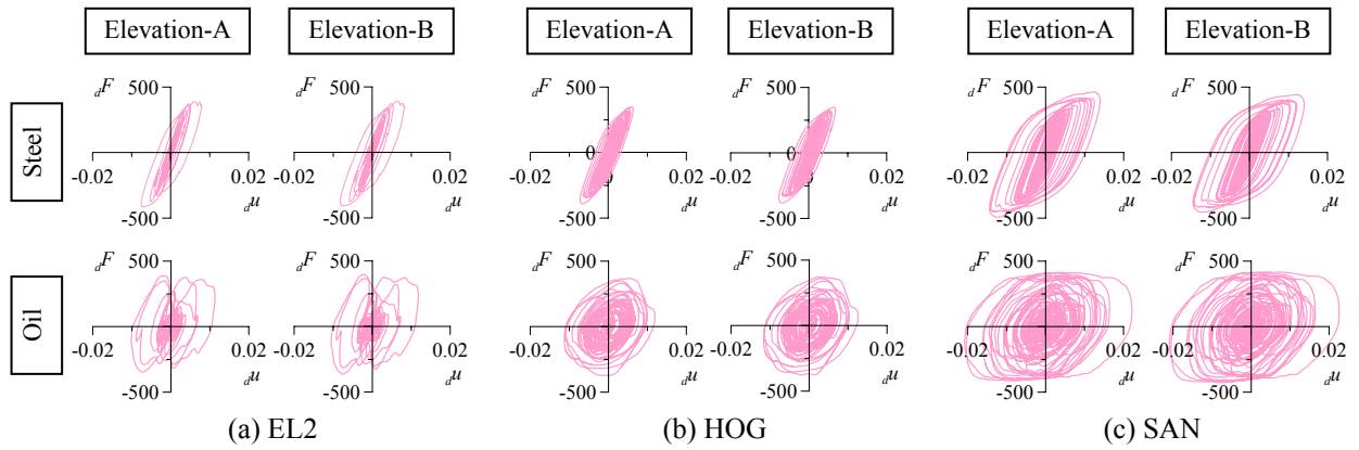
Figure 7. 2 nd story damper deformation – force relationship ( unit : kN, m )
