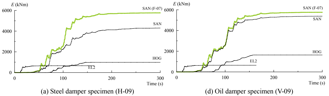
Figure 10. Time history of input energy
