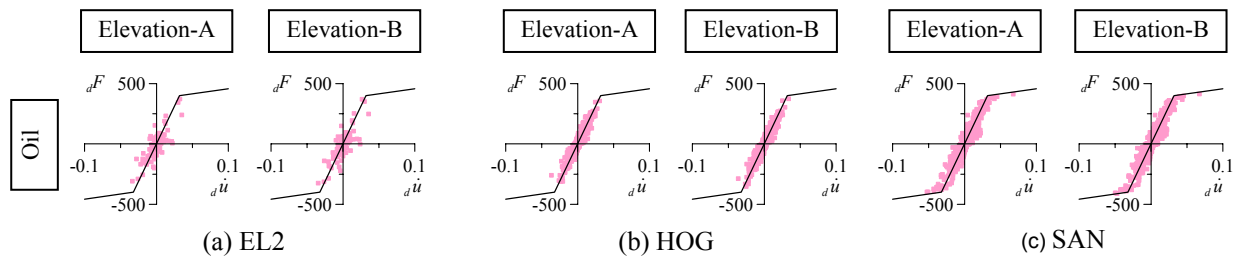
Figure 8. 2 nd story oil-damper velocity – force relationship ( unit : kN, m/s )
