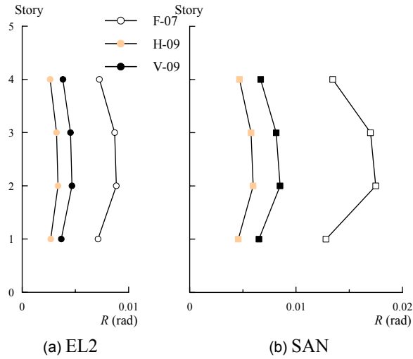
Figure 5. Maximum inter-story drift angle
