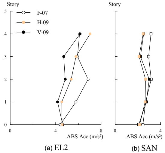
Figure 6. Maximum acceleration
