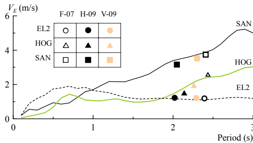
Figure 11. V_E - spectrum vs. test results (plots)
