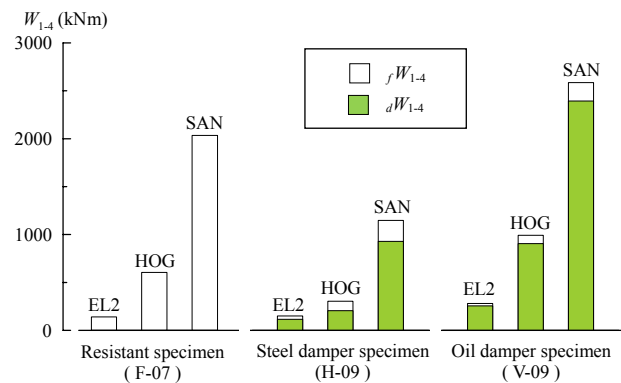
Figure 15. Energy distribution in lower moment frame
