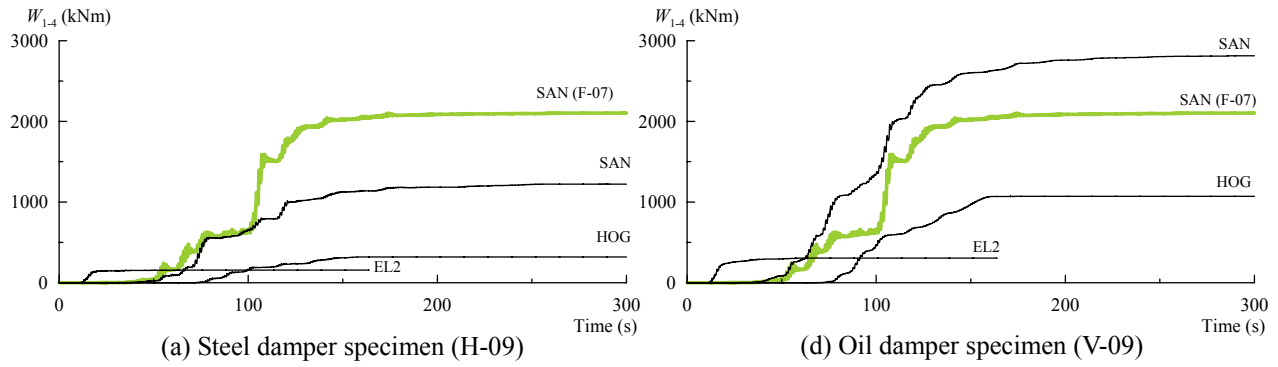
Figure 14. Time history of input energy for the moment frame
