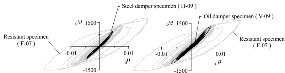
Figure 13. Beam Moment – rotation relationship ( unit : kN/m, rad )
