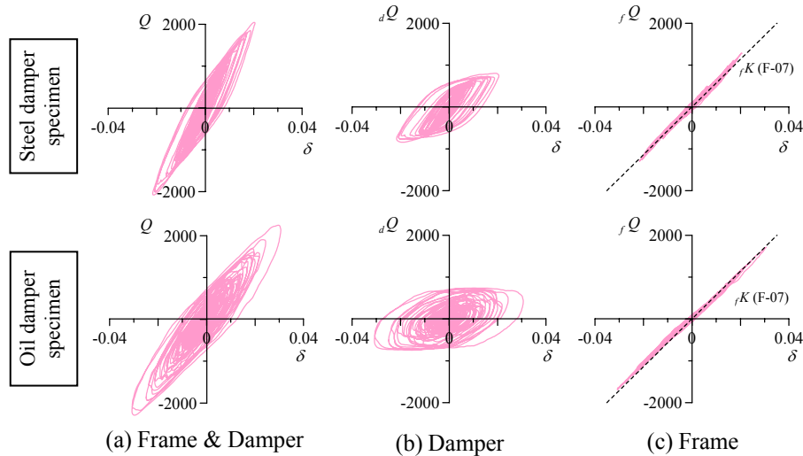
Figure 12. 2 nd story deformation – force relationship ( unit : kN, m )
