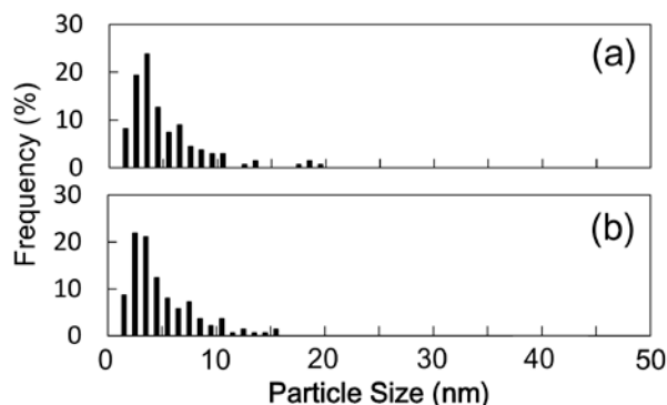
Figure 7. Particle size distributions of silicon nanoparticles. (Irradiation time: (a) 1 hour and (b) 3 hours. Energy density: 0.17 J/cm².)
