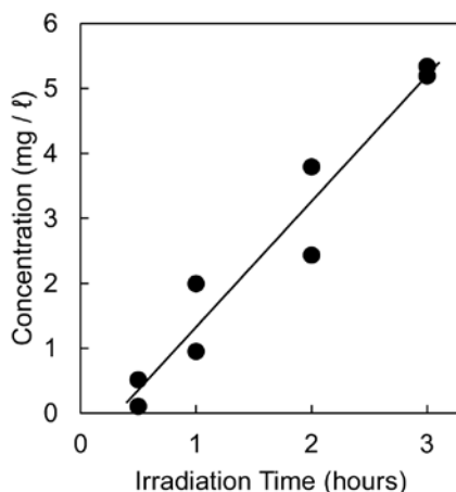
Figure 8. Silicon nanoparticle quantity as a function of irradiation time.
