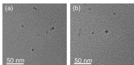
Figure 6. TEM images of silicon nanoparticles. (Irradiation time: (a) 1 hour and (b) 3 hours. Energy density: 0.17 J/cm².)
