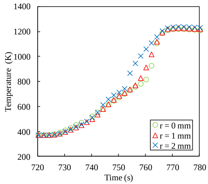
Figure 3.4 Temperature histories at three locations within the wood cylinder during the pyrolysis at heating rate of 30 K/s.
