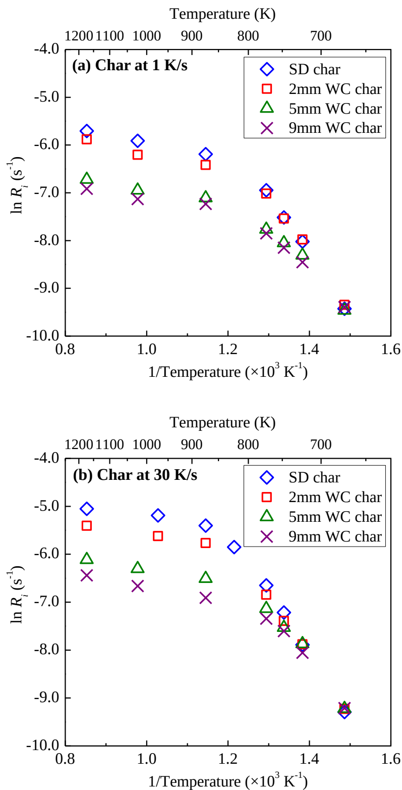
Figure 3.14 Arrhenius plot of reactivity for chars prepared at heating rates of (a) 1 K/s and (b) 30 K/s.
