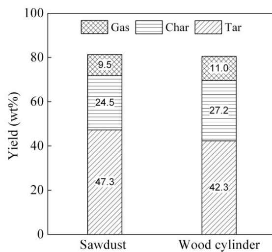
Figure 2.11 Total product yields for the sawdust and wood cylinder.
