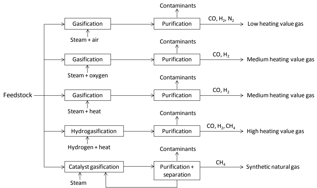
Figure 1.10 Gasification methods [33].
