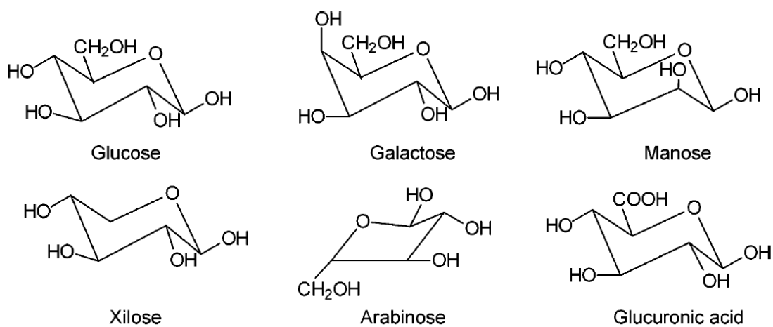
Figure 1.7 Main components of hemicelluloses [19].
