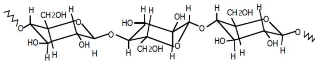
Figure 1.6 Molecular structure of cellulose.
