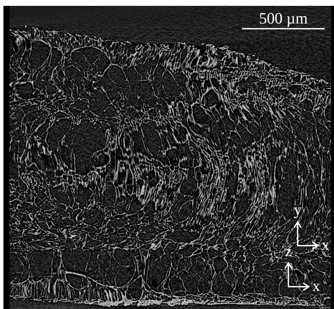
Figure 4.3 X-ray CT cross-sectional image of D8×L2 char in the xz plane.
