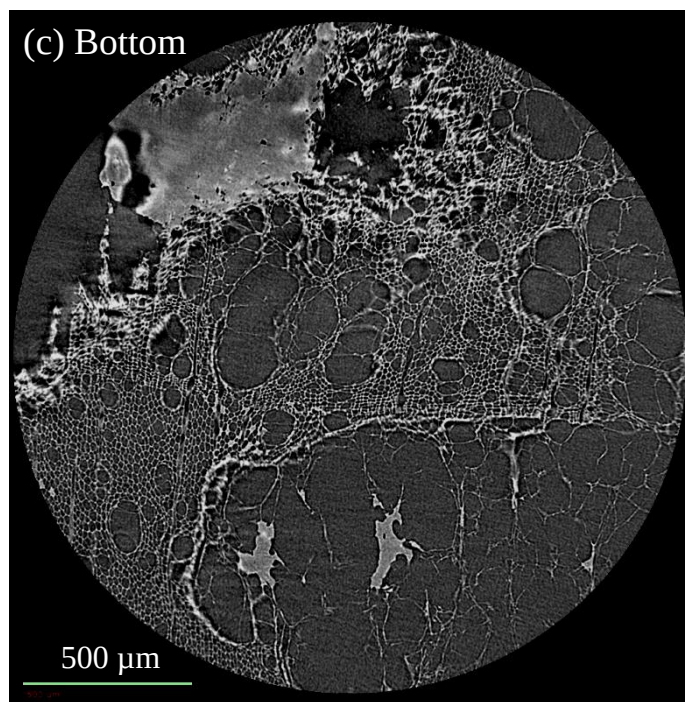
Figure 4.2 X-ray CT cross-sectional image of D8×L2 char in the xy plane: (a) near top surface, (b) at the middle, and (c) near bottom surface.
