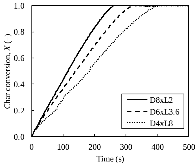
Figure 4.12 Char conversion as a function of time at gasification temperature 1423K. Chars are prepared at heating rate 1 K/s.
