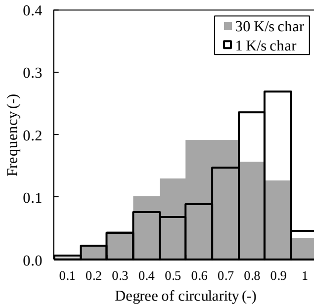
Figure 3.11 Distributions of the degree of circularity of pore for the chars prepared at 1 and 30 K/s.
