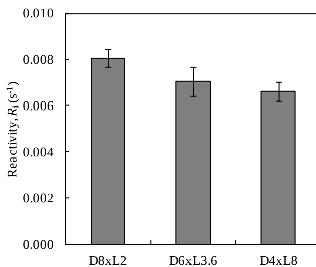
Figure 4.6 Reactivity of three aspect ratio chars prepared at 30 K/s. Gasification temperature is 1423K. Error bars indicate one standard deviation.
