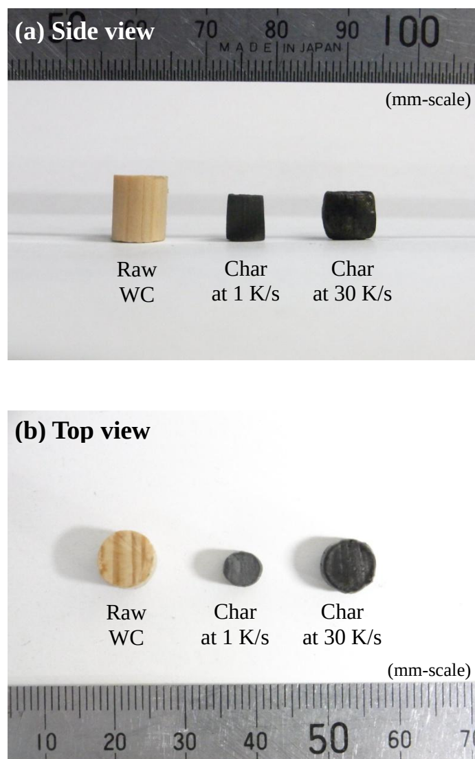
Figure 3.12 Photographs of raw material of wood cylinder and wood cylinder chars prepared at heating rates of 1 and 30 K/s (left to right) captured from (a) side view and (b) top view.
