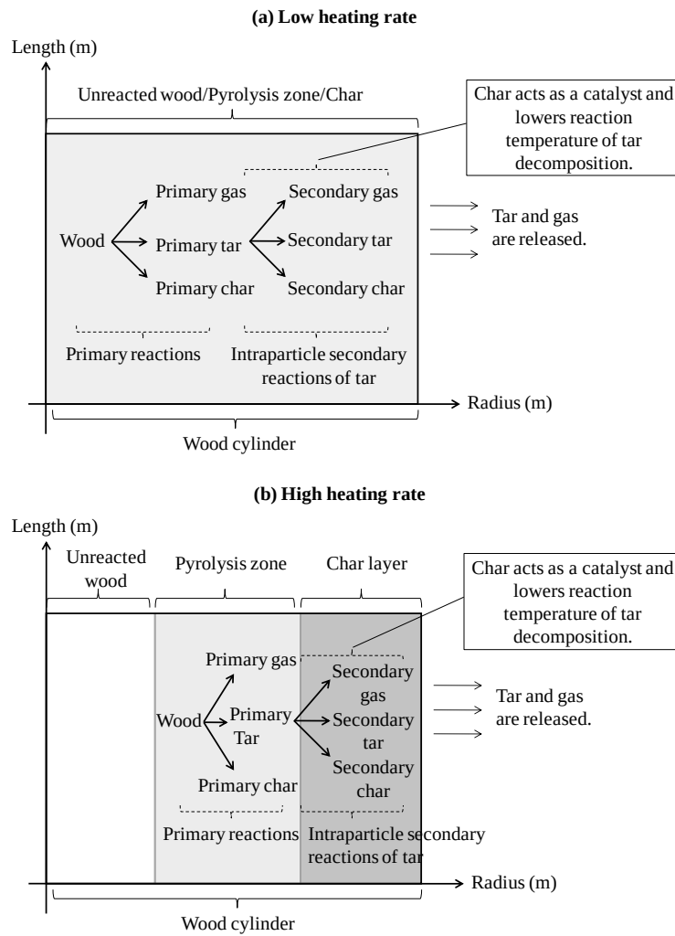
Figure 2.16 Mechanism diagram of the intraparticle secondary reactions of tar: (a) at low heating rate and (b) at high heating rate.
