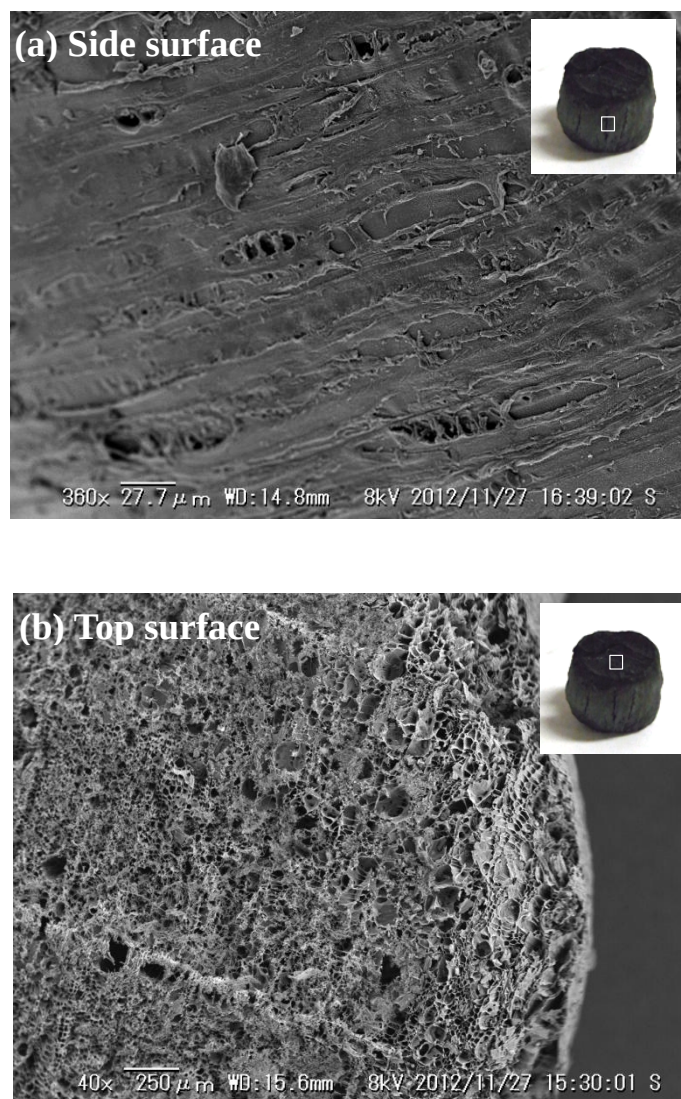
Figure 3.7 SEM images of (a) side surface and (b) top surface of 9 mm wood cylinder char prepared at heating rate of 30 K/s.
