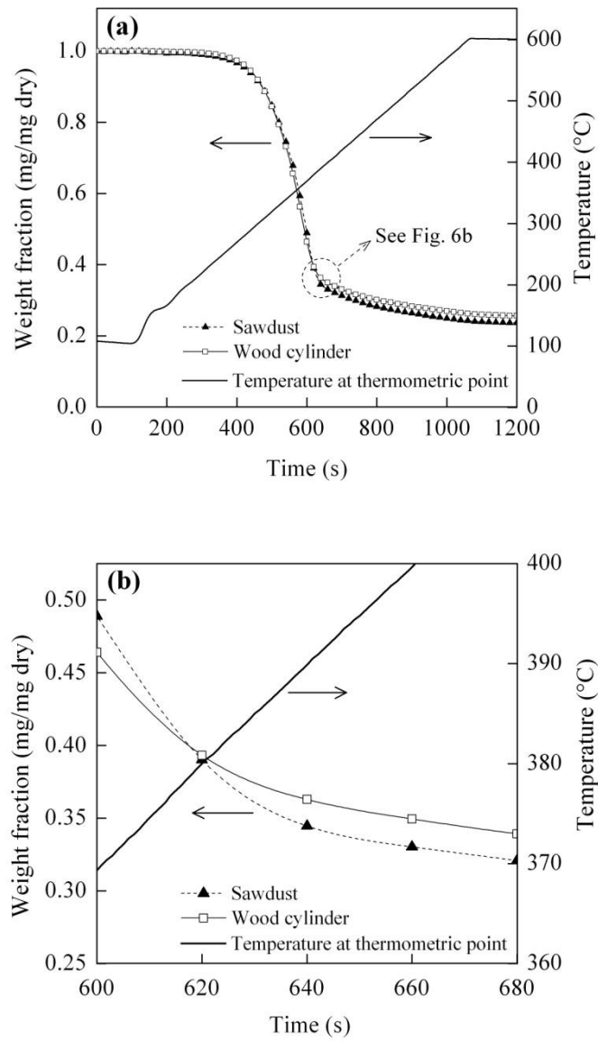
Figure 2.8 Weight fraction histories of the sawdust and wood cylinder, along with the thermometric temperature: (a) for entire pyrolysis and (b) for 600–680 s.
