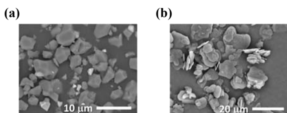
Fig. 1. SEM images of (a) AlN and (b) hBN particles
