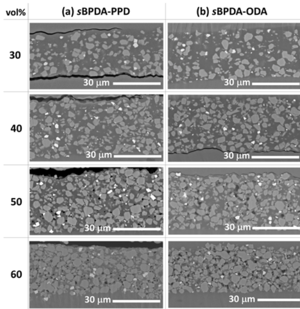
Fig.1 Cross-sectional SEM images of AlN/PI films. (a) AlN/sBPPD and (b) AlN/sBPOD
