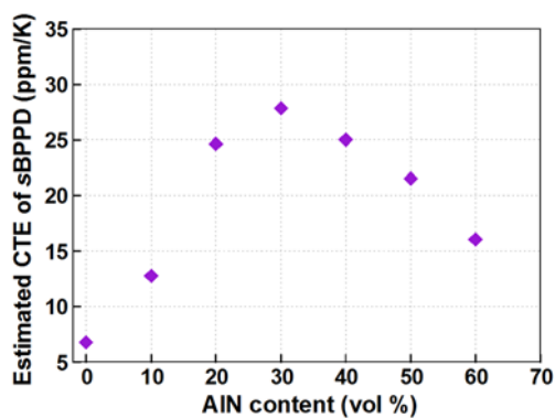
Fig.10 Estimated CTE of sBPPD matrix in the presence of AlN particles
