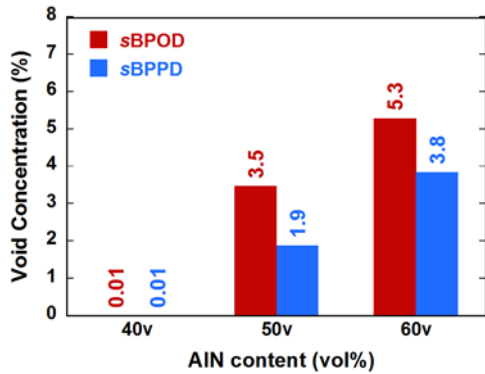
Fig. 2 The void concentration ( \phi_v ) of 40v to 60v-AlN/PI.
