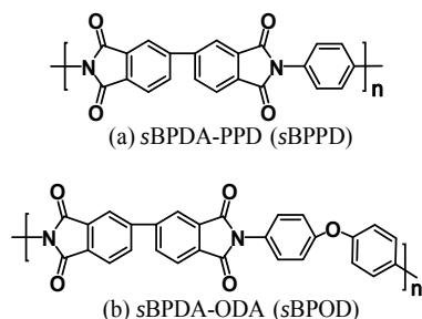
Scheme 1. Chemical structures of PI matrices.
