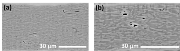
Fig.4 Cross-sectional SEM images of (a) 40v-hBN/sBPPD and 40v-hBN/sBPOD.
