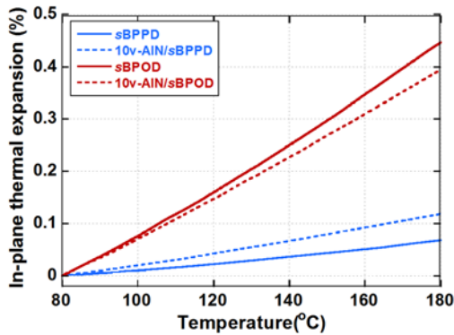
Fig.7 TMA curves of pristine PIs and 10v-AIN/PIs.
