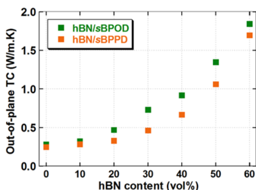
Fig.5 Out-of-plane thermal conductivities of hBN/PI films.
