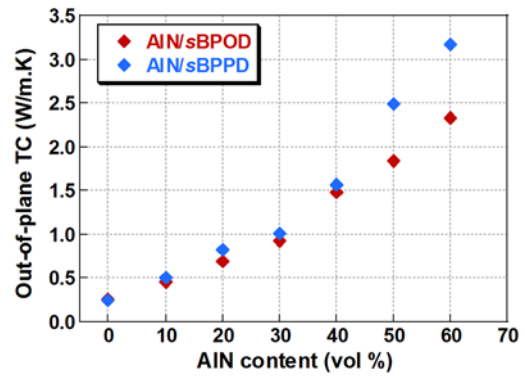
Fig.3 Out-of-plane thermal conductivities of AlN/PI films.
