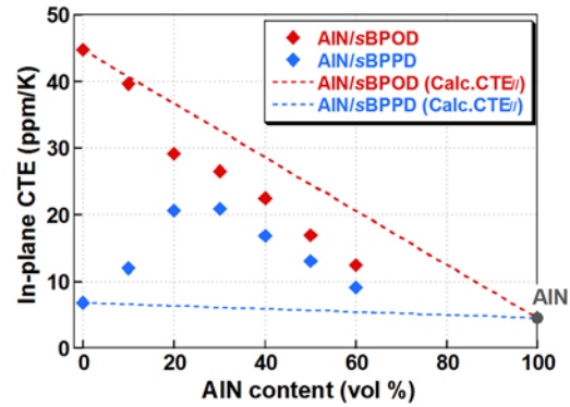
Fig.8 In-plane CTEs of AIN/PI films (80–180 °C).
