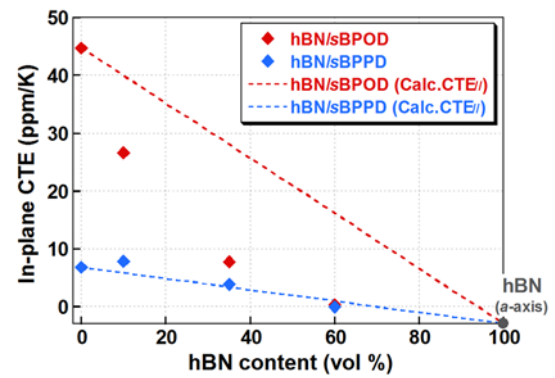
Fig.9 In-plane CTEs of hBN/PI films (80–180 °C).
