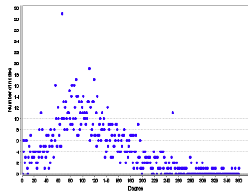
Figure 7 Items' Degree Distribution
