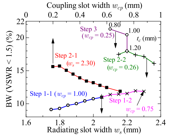
Fig. 5 Reflection bandwidth improvement.
