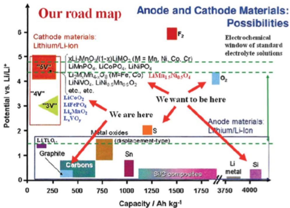
Figure 1.2 A review of advanced and practical lithium battery materials [14].
