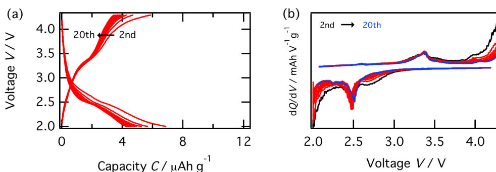
Figure 3.9 (a) Charge-discharge and (b) dQ/dV curves of \text{SrTiO}_3 (100) substrate where gold is coated.
