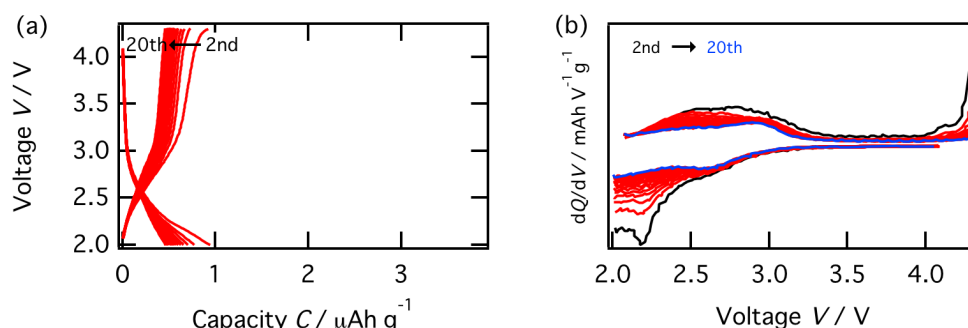
Figure 3.8 (a) Charge-discharge and (b) dQ/dV curves of \text{SrTiO}_3 (100) substrate at a range between 2.0 and 4.3 V.
