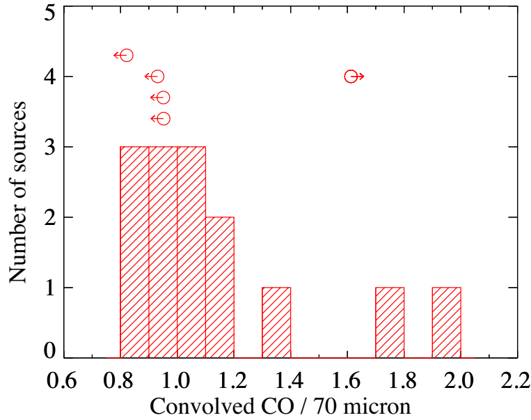
FIGURE 3.5: The histogram of the ratio of the convolved CO radius to the HWHM of MIPS 70\mu\text{m} is shown. The CO radius s_A in the Gaussian model is used and is convolved by the Gaussian with the same FWHM as one of the PSF of MIPS 70\mu\text{m} , 18'' . The average ratio is 1.0 and the standard deviation is 0.1 except for IC2810W, MCG+04-48-002S and Mrk 331 whose ratios are larger than 1.3. Two sources, IC 1623AB and IRAS F14348-1447, are not included in the histogram because of no available data of MIPS 70\mu\text{m} image. The upper or lower limits of the ratio are also plotted as the arrows above the histogram.
