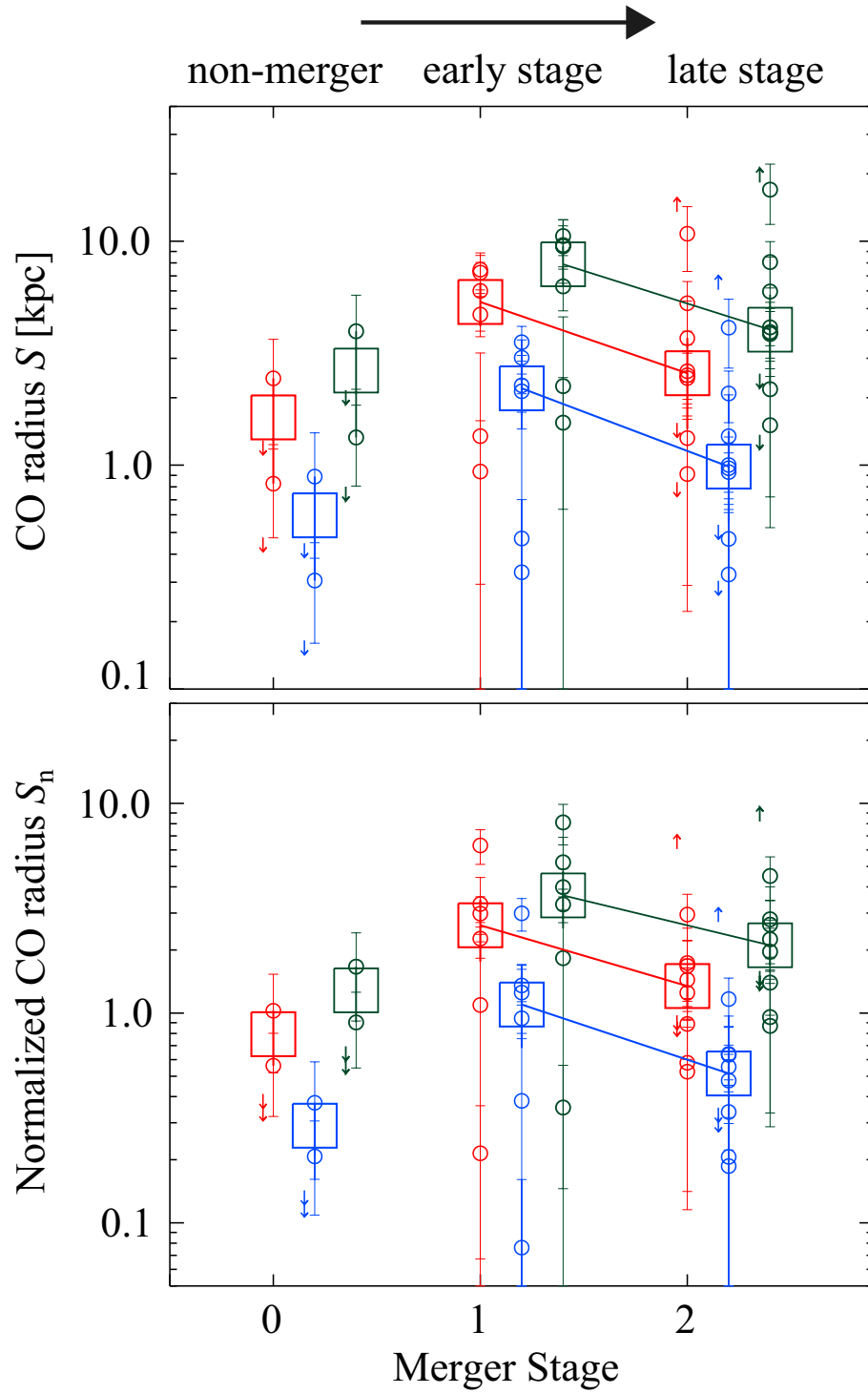
FIGURE 3.6: The CO size (a) and the normalized CO size (b) at the each merger stage of the sub-sample. The each of the CO size and the normalized CO size are colored the same color scheme as Figure 3.3 and are slightly shifted in one merger stage. The circles, fine vertical bars and arrows mean the data values, the errors and the upper/lower limit values, respectively. The squares and the vertical bold bars are the median values and its error, respectively.
