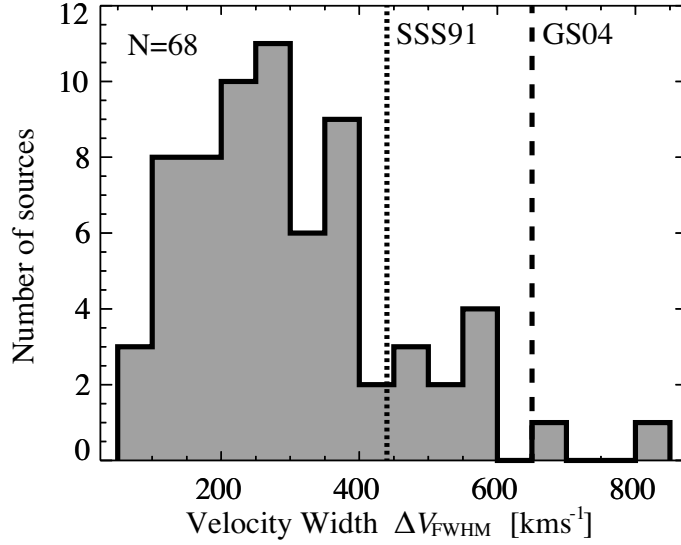
FIGURE 2.7: The histogram of the velocity width \Delta V_{\text{FWHM}} of CO line. The average value is 300 kms ^{-1} . The maximum is 840 kms ^{-1} of UGC 05101. A vertical dotted line and a dashed line represent maximum values observed by SSS91 and GS04, respectively.
