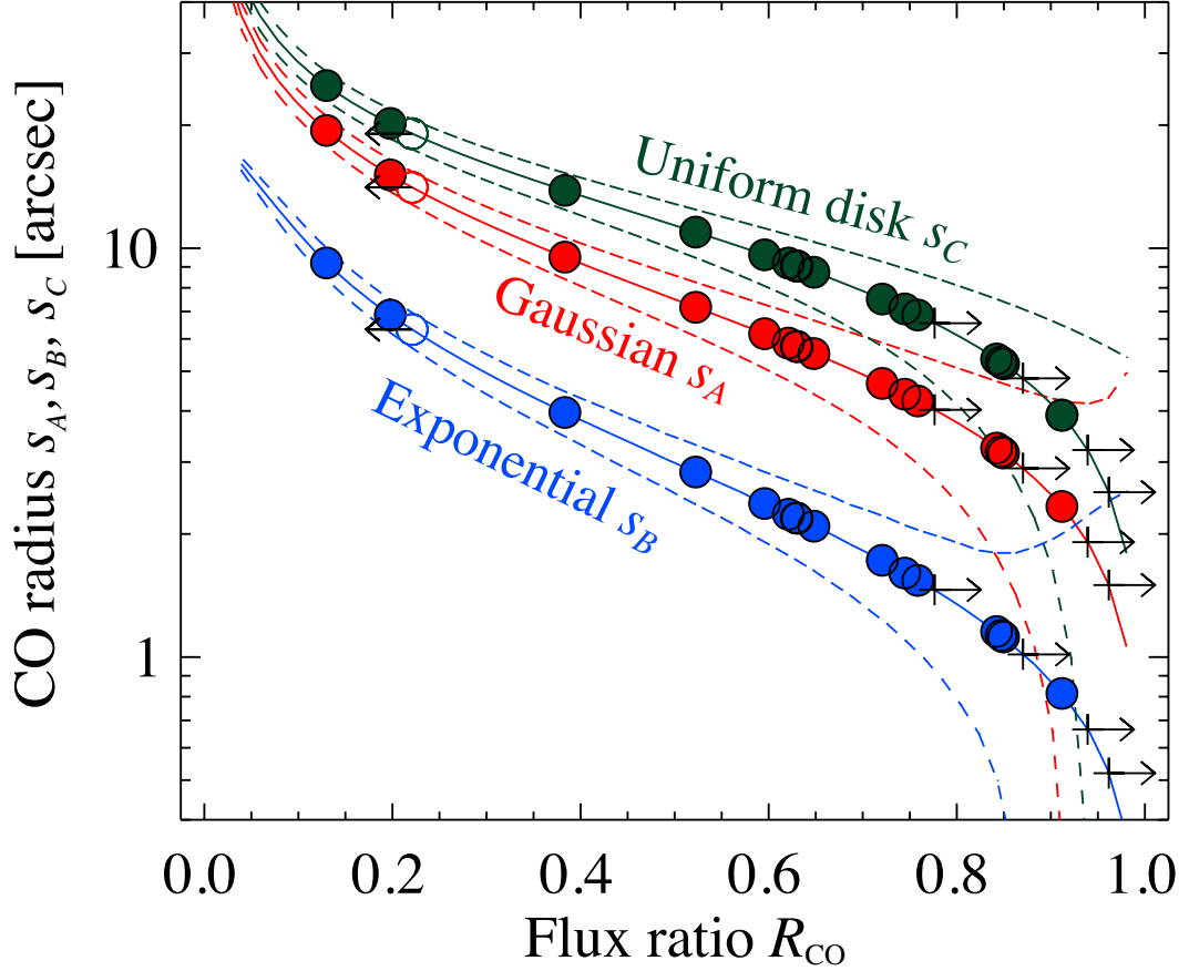
FIGURE 3.3: The angular CO radius s and the flux ratio ( R_{CO} ) of the sub-sample which can be estimated (see text). The CO radius s in y-axis represents s_A for the Gaussian model (Model A, red) and s_B for the exponential model (Model B, blue), and s_C for the radius for the uniform disk model (Model C, green). The solid and the dashed lines indicate the model curve of A, B and C, respectively. The right (left) arrow denotes the lower limit (upper limit) of R_{CO} and the upper limit (lower limit) of s .
