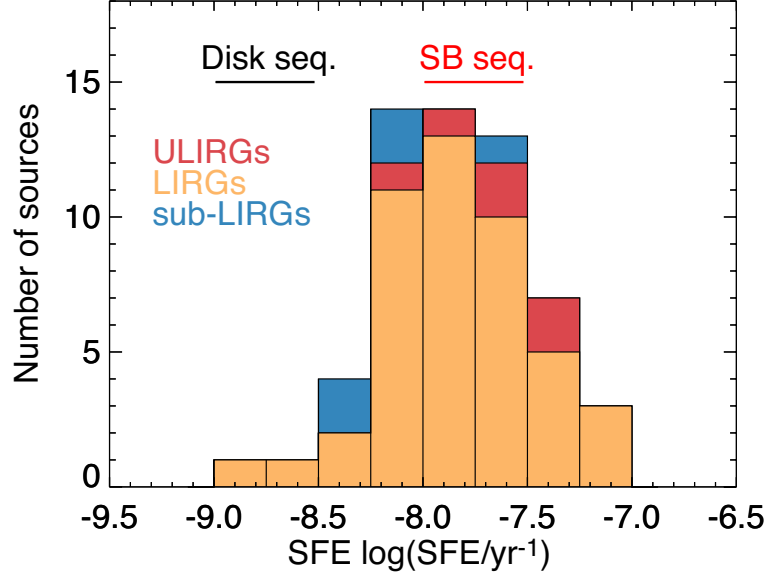
FIGURE 4.4: The SFE in the central regions of the sample. The SFE is defined in Equation 4.4. The SFR is estimated from the Equation 4.3 using the 24\mu\text{m} luminosity and the AGN contributions are corrected. The molecular gas mass is from our CO observations. The ULIRGs, LIRGs and sub-LIRGs are shown by red, orange and blue boxes, respectively. The SFE ranges from 1.8 \times 10^{-9} \text{ yr}^{-1} to 72 \times 10^{-9} \text{ yr}^{-1} , with a median of 14 \times 10^{-9} \text{ yr}^{-1} and with an average of 19 \times 10^{-9} \text{ yr}^{-1} . The red and black solid lines represent the expected SFEs of a galaxy with a IR luminosity of 10^{11-13} L_{\odot} on the each modes of the starburst sequence and the disk star-formation sequence (Daddi et al., 2010a).
